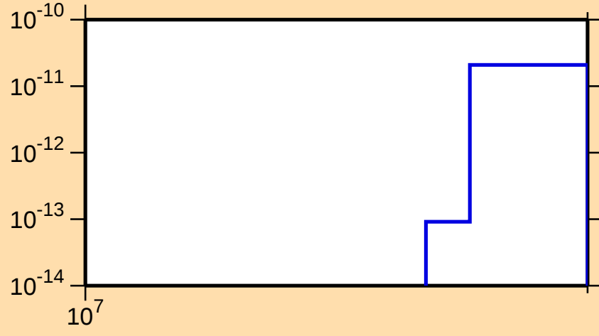
\sigma vs. E for ^{246}\text{Bk}(n,3n\alpha)
