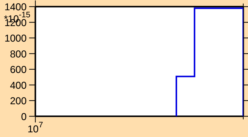
\sigma vs. E for ^{246}\text{Bk}(n,p\alpha)
