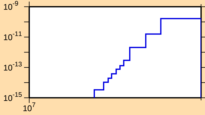
\sigma vs. E for ^{246}\text{Bk}(n,\text{He3})
