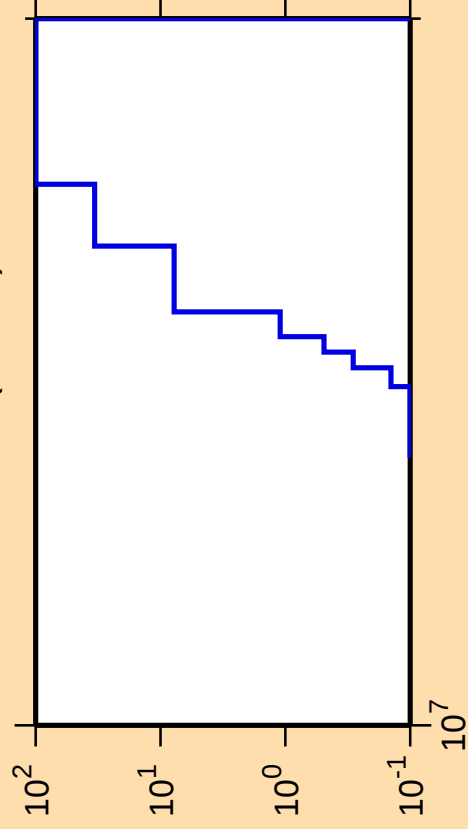
\Delta\sigma/\sigma vs. E for ^{246}\text{Bk}(n,\text{He3})
