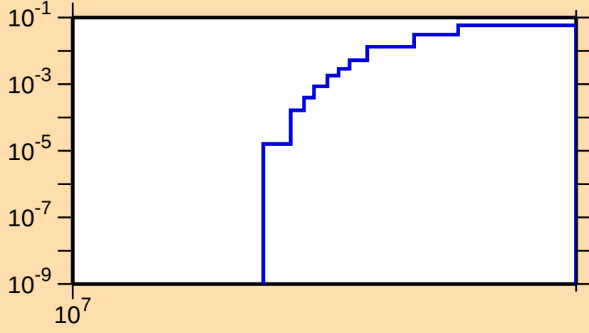
\sigma vs. E for ^{246}\text{Bk}(n,3n)
