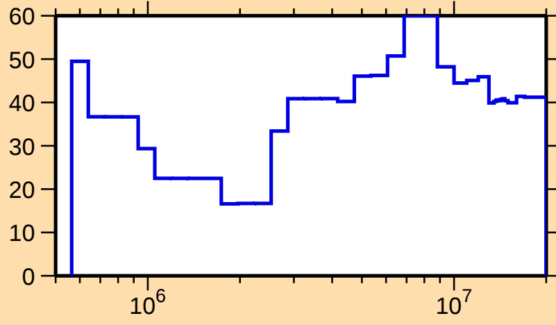
\Delta\sigma/\sigma vs. E for ^{246}\text{Bk}(n,n\text{cont.})
