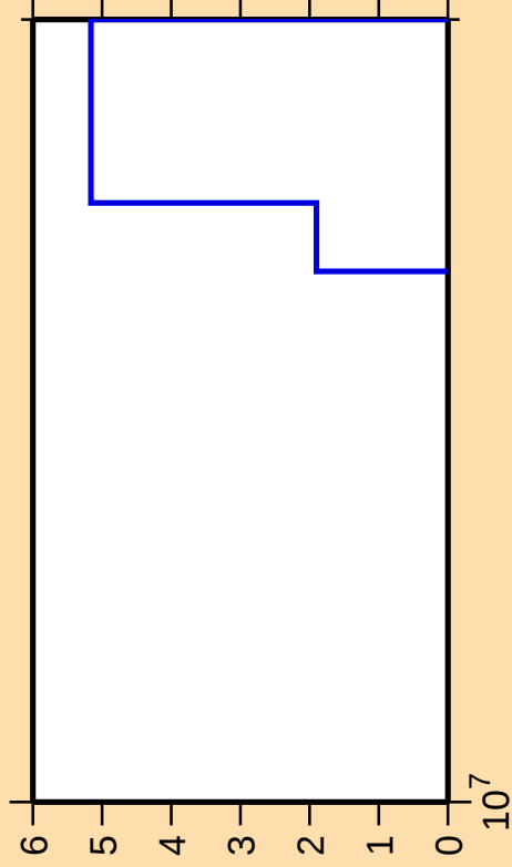
\Delta\sigma/\sigma vs. E for ^{246}\text{Bk}(n,p\alpha)
