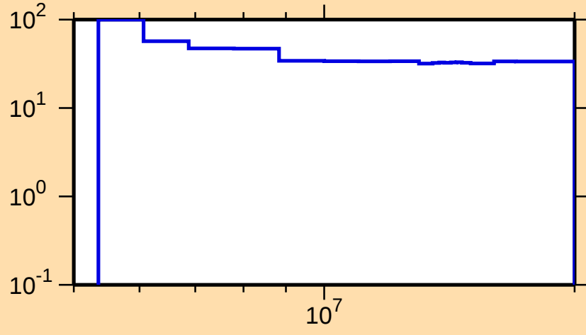
\Delta\sigma/\sigma vs. E for ^{251}\text{Bk}(n,2n)
