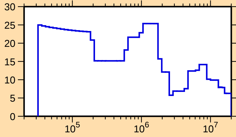
\Delta\sigma/\sigma vs. E for ^{251}\text{Bk}(n,\text{el.})
