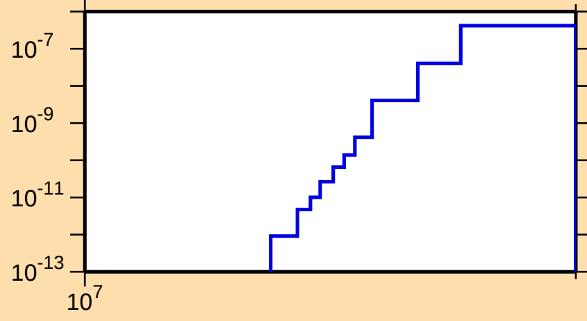
\sigma vs. E for ^{251}\text{Bk}(n,\text{nd})
