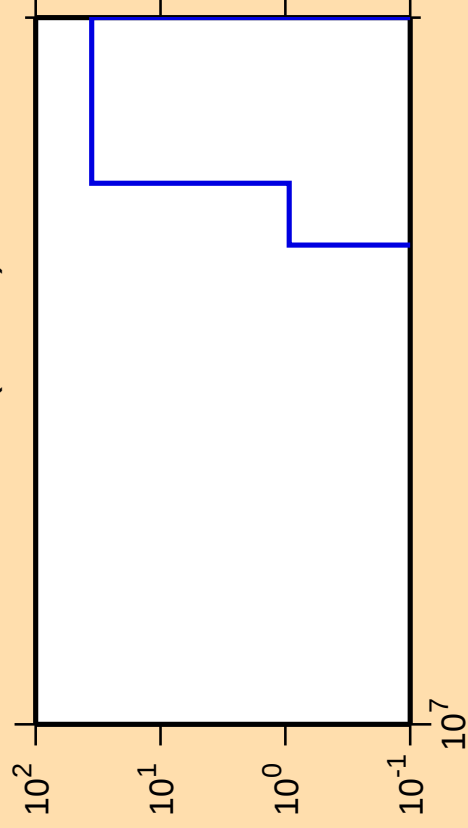
\Delta\sigma/\sigma vs. E for ^{251}\text{Bk}(n,\text{He3})
