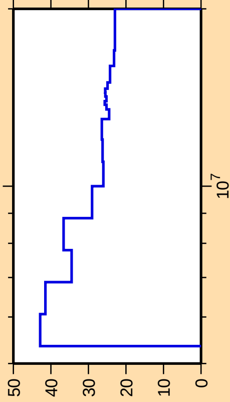
\Delta\sigma/\sigma vs. E for ^{251}\text{Bk}(n,n\text{cont.})
