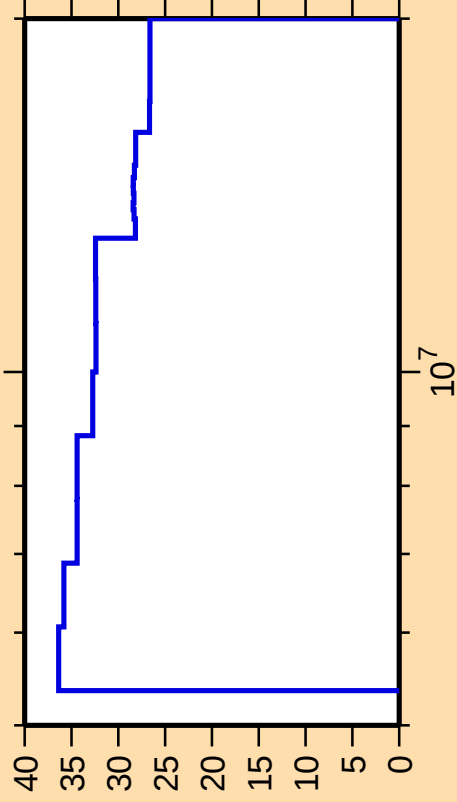
\Delta\sigma/\sigma vs. E for ^{251}\text{Bk}(n,n_1)
