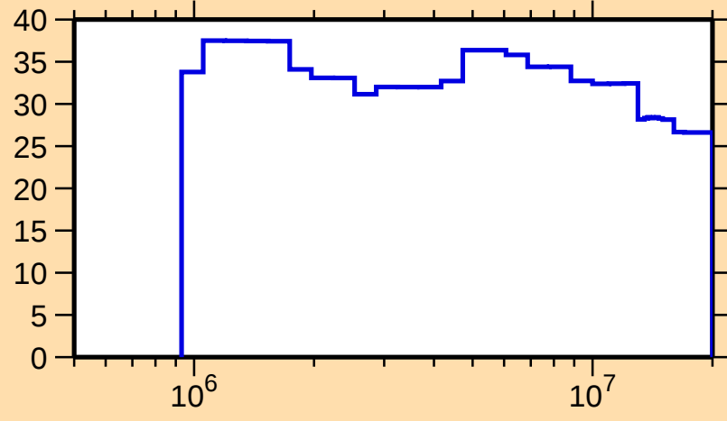
\Delta\sigma/\sigma vs. E for ^{251}\text{Bk}(n,n_1)
