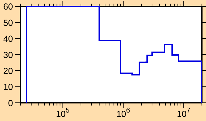
\Delta\sigma/\sigma vs. E for ^{251}\text{Bk}(n,\text{inel.})
