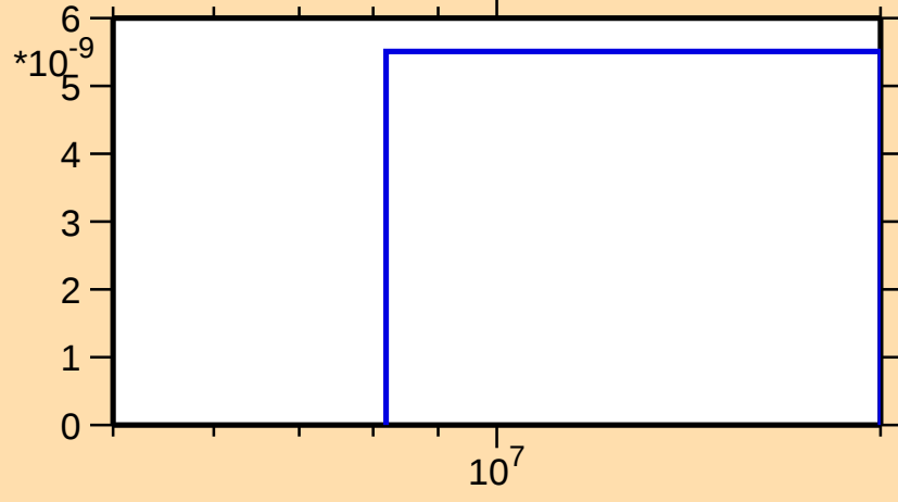
\sigma vs. E for ^{251}\text{Bk}(n,nd)
