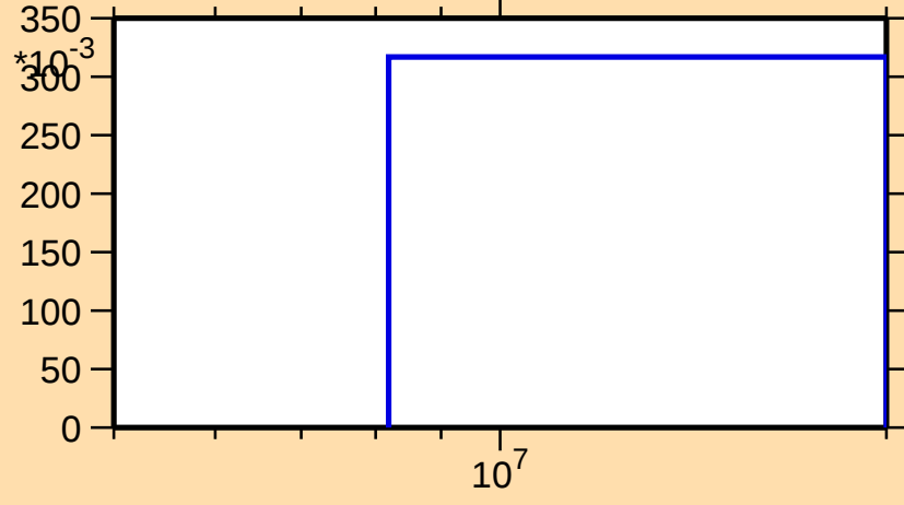
\sigma vs. E for ^{251}\text{Bk}(n,3n)
