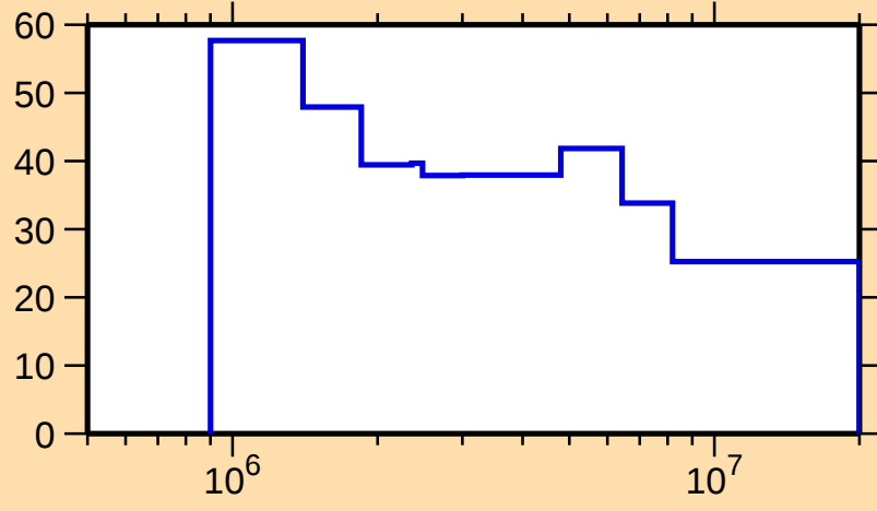
\Delta\sigma/\sigma vs. E for ^{251}\text{Bk}(n,n\text{cont.})
