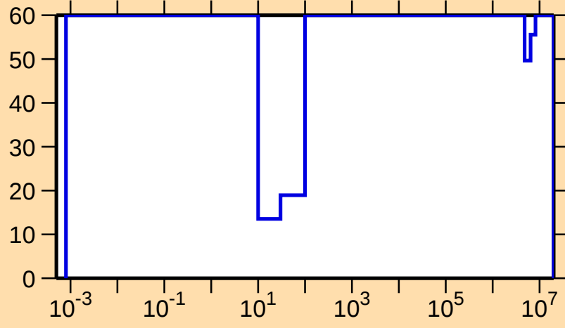
\Delta\sigma/\sigma vs. E for ^{251}\text{Bk}(n,\gamma)
