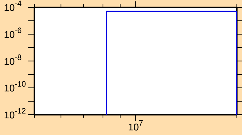
\sigma vs. E for ^{251}\text{Bk}(n,np)
