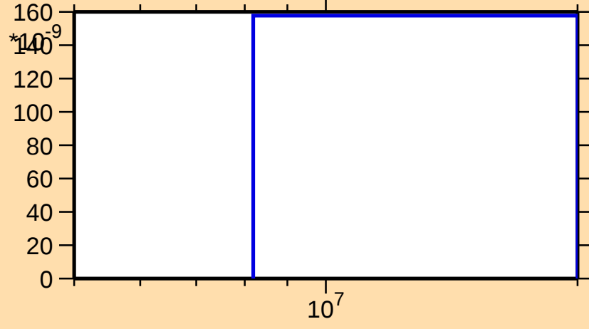
\sigma vs. E for ^{251}\text{Bk}(n,nt)
