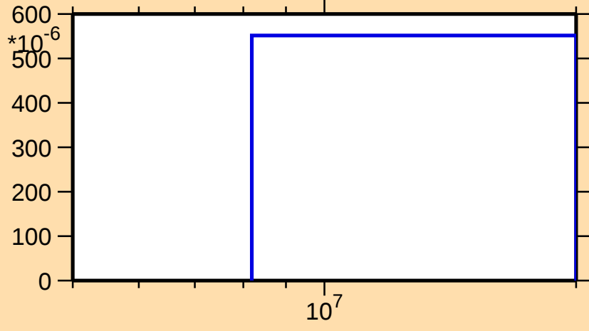
\sigma vs. E for ^{72}\text{Br}(n,\text{pd})
