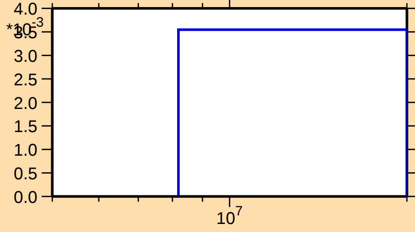
\sigma vs. E for ^{72}\text{Br}(n,2n)
