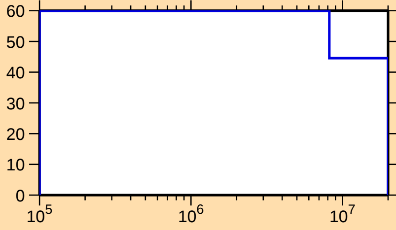
\Delta\sigma/\sigma vs. E for ^{72}\text{Br}(n,n\text{cont.})
