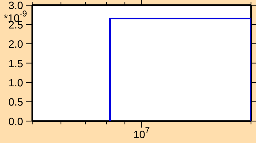
\sigma vs. E for ^{72}\text{Br}(\text{mt } 34)
