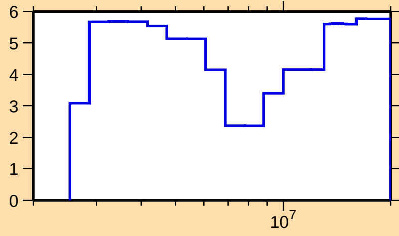
\Delta\sigma/\sigma vs. E for ^{84}\text{Br}(\text{n},\text{el.})
