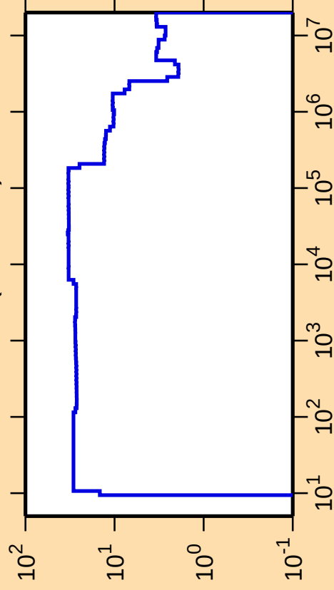
\Delta\sigma/\sigma vs. E for ^{84}\text{Br}(n,\text{nonel.})
