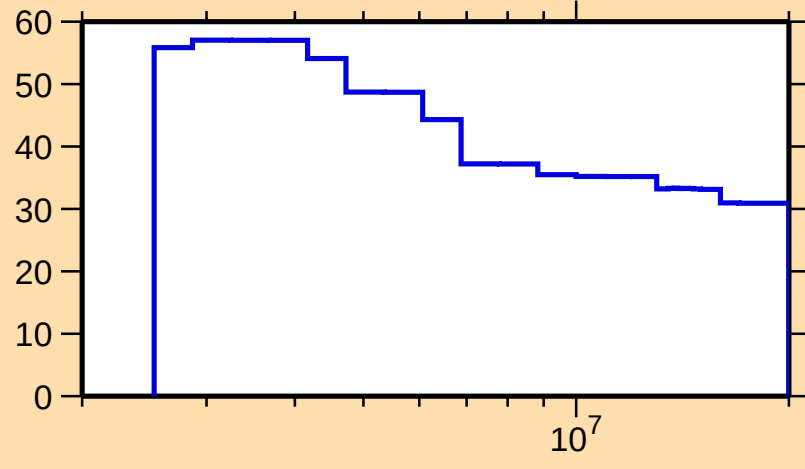
\Delta\sigma/\sigma vs. E for ^{84}\text{Br}(n,p)
