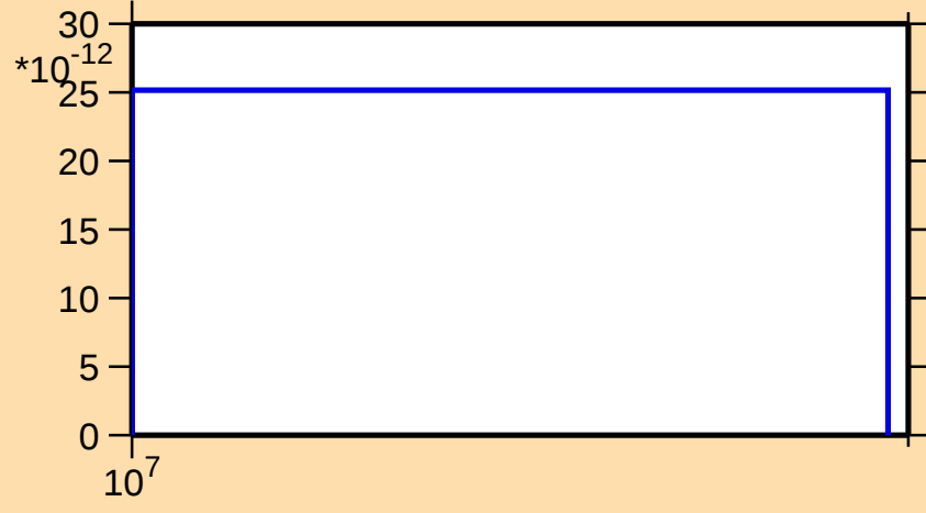
\sigma vs. E for ^{84}\text{Br}(n,\text{nt})
