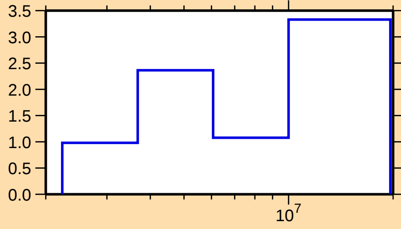
\Delta\sigma/\sigma vs. E for ^{84}\text{Br}(\text{n},\text{tot.})
