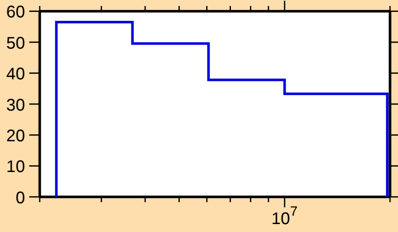
\Delta\sigma/\sigma vs. E for ^{84}\text{Br}(n,p)
