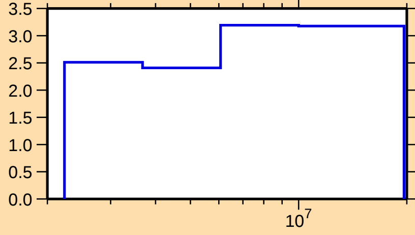
\Delta\sigma/\sigma vs. E for ^{84}\text{Br}(\text{n},\text{nonel.})
