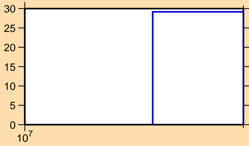
\Delta\sigma/\sigma vs. E for ^{14}\text{C}(n,ncont.)
