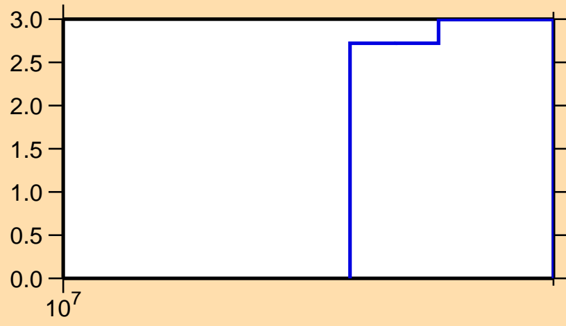
\Delta\sigma/\sigma vs. E for ^{14}\text{C}(n,n\text{onel.})
