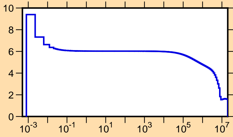
\sigma vs. E for ^{14}\text{C}(n,\text{tot.})
