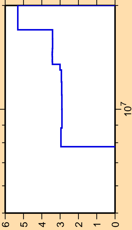
\Delta\sigma/\sigma vs. E for ^{14}\text{C}(n,n_3)
