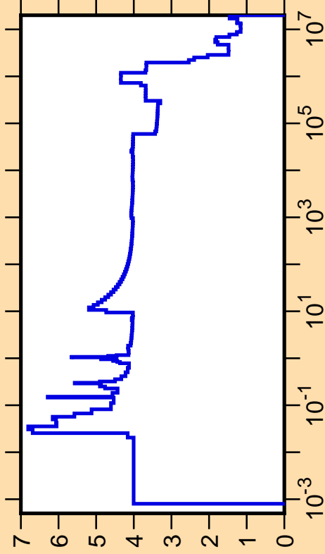
\Delta\sigma/\sigma vs. E for ^{14}\text{C}(n,\text{tot.})
