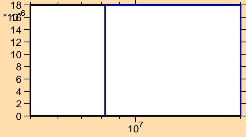
\sigma vs. E for ^{104}\text{Cd}(n,t)
