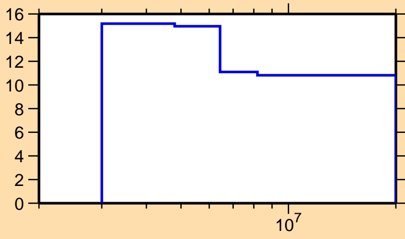
\Delta\sigma/\sigma vs. E for ^{104}\text{Cd}(n,n\text{cont.})
