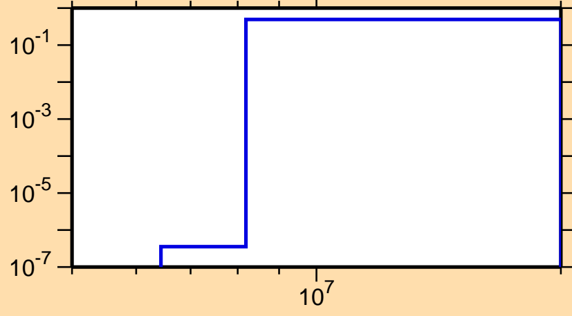
\sigma vs. E for ^{104}\text{Cd}(n,np)
