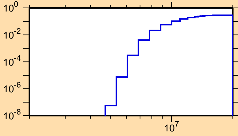
\sigma vs. E for ^{123}\text{Ce}(n,np)
