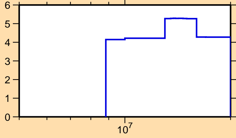
\Delta\sigma/\sigma vs. E for ^{125}\text{Ce}(n,\text{nonel.})
