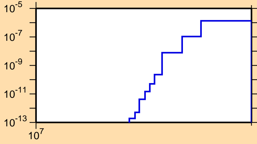
\sigma vs. E for ^{125}\text{Ce}(n,\text{nd})
