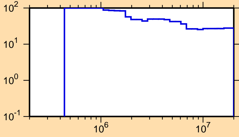
\Delta\sigma/\sigma vs. E for ^{125}\text{Ce}(n,\text{inel.})
