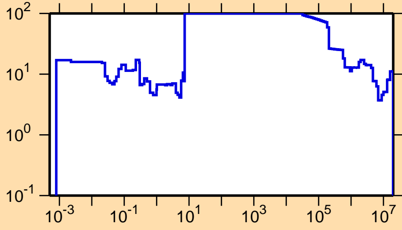
\Delta\sigma/\sigma vs. E for ^{125}\text{Ce}(n,\text{tot.})
