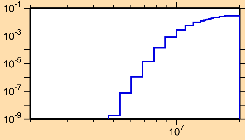
\sigma vs. E for ^{125}\text{Ce}(n,d)
