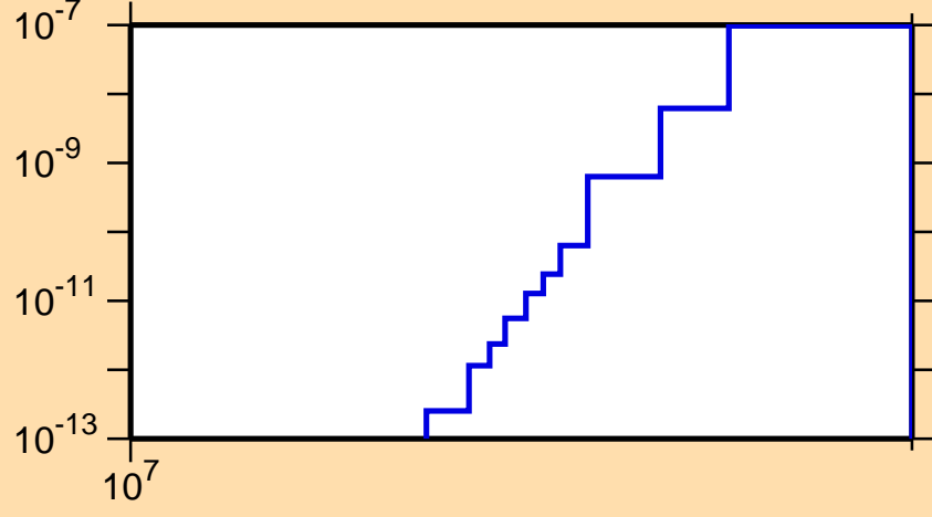
\sigma vs. E for ^{125}\text{Ce}(\text{mt } 34)
