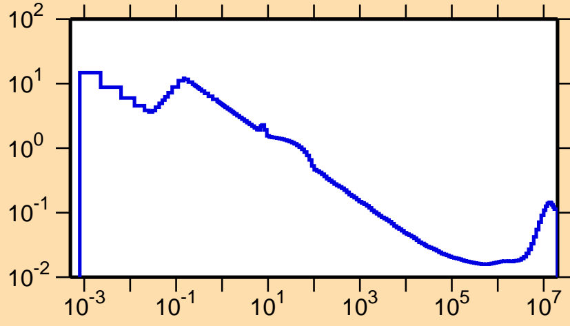
\sigma vs. E for ^{125}\text{Ce}(n,\alpha)
