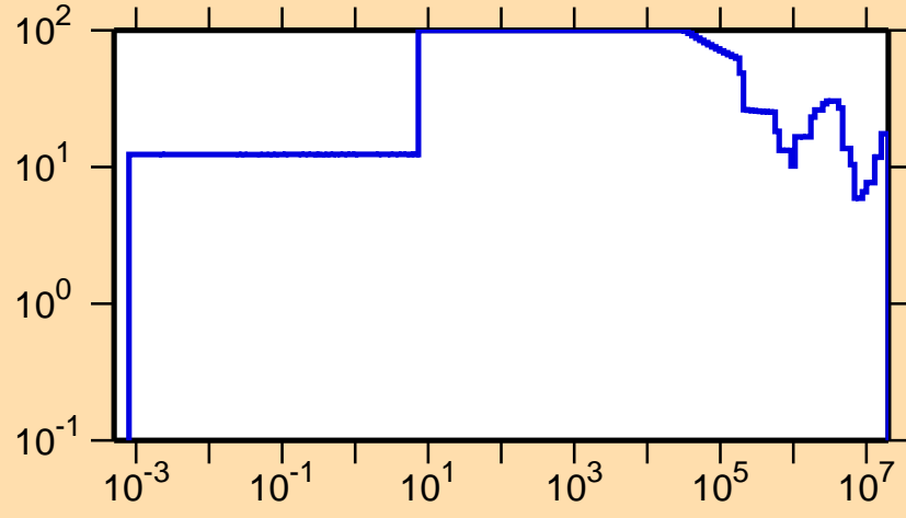
\Delta\sigma/\sigma vs. E for ^{125}\text{Ce}(n,\text{el.})
