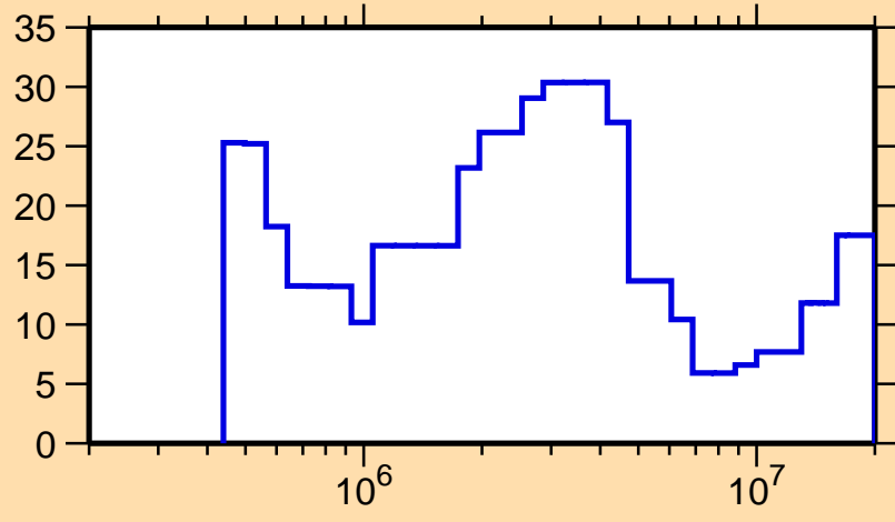
\Delta\sigma/\sigma vs. E for ^{125}\text{Ce}(n,\text{el.})
