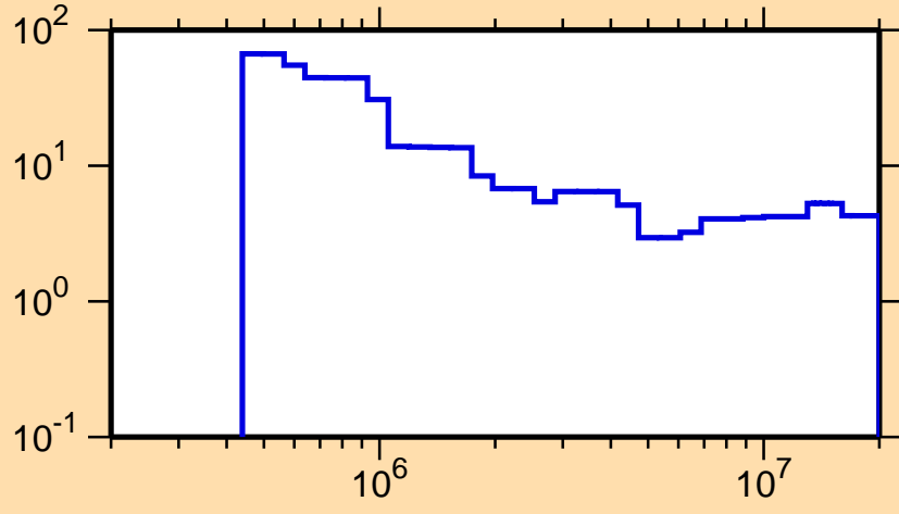
\Delta\sigma/\sigma vs. E for ^{125}\text{Ce}(n,\text{nonel.})
