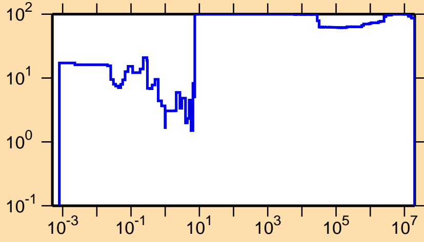
\Delta\sigma/\sigma vs. E for ^{125}\text{Ce}(n,\gamma)
