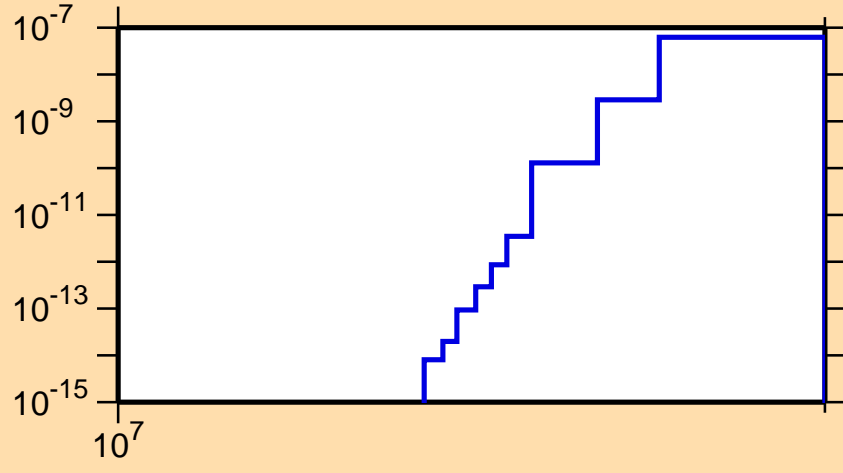
\sigma vs. E for ^{125}\text{Ce}(n,2n\alpha)
