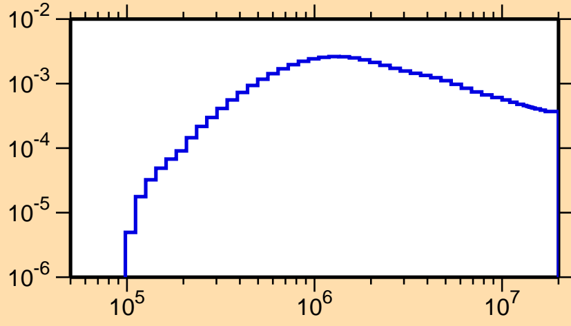
\sigma vs. E for ^{125}\text{Ce}(n,n_1)
