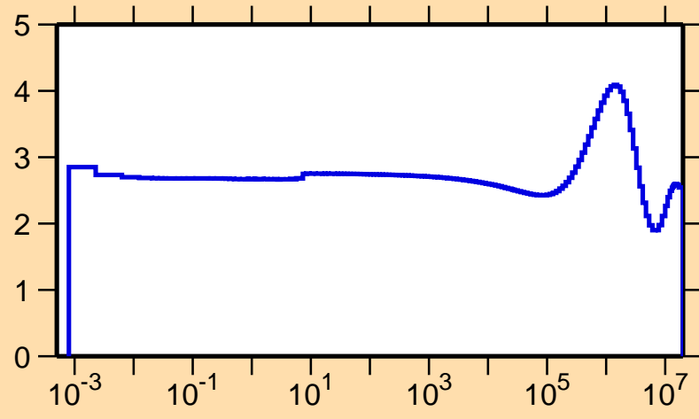
\sigma vs. E for ^{125}\text{Ce}(n,\text{el.})
