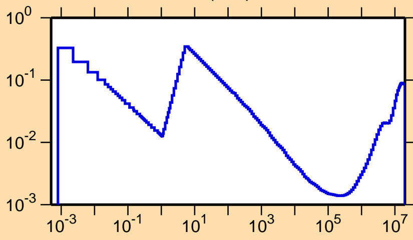
\sigma vs. E for ^{126}\text{Ce}(n,\alpha)
