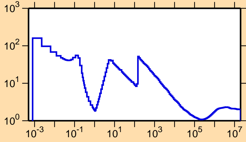
\sigma vs. E for ^{126}\text{Ce}(n,\text{nonel.})
