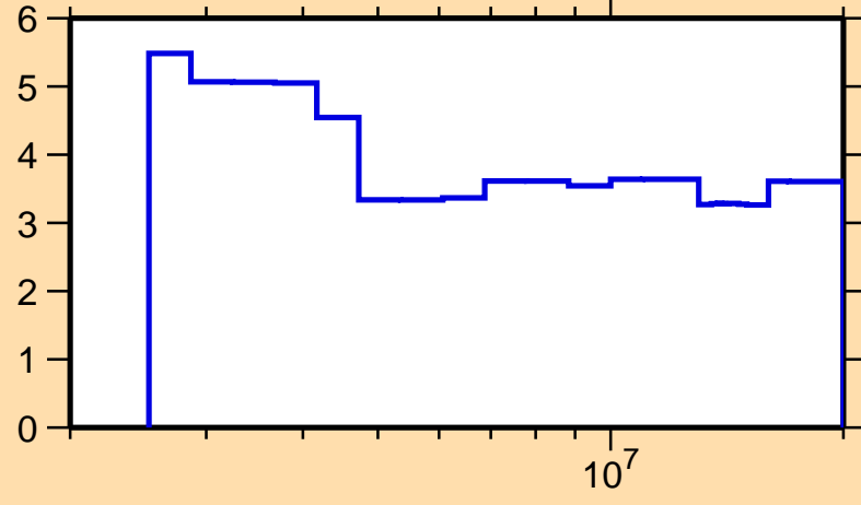
\Delta\sigma/\sigma vs. E for ^{130}\text{Ce}(n,\text{nonel.})
