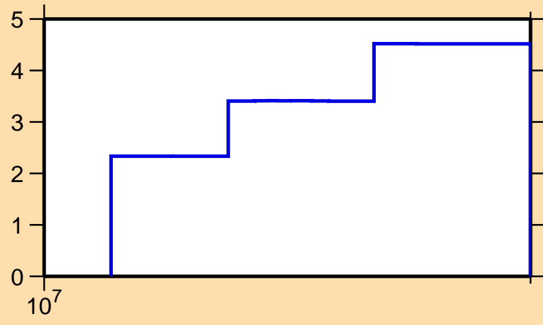
\Delta\sigma/\sigma vs. E for ^{130}\text{Ce}(n,\text{tot.})
