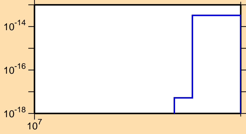
\sigma vs. E for ^{130}\text{Ce}(n,nt)
