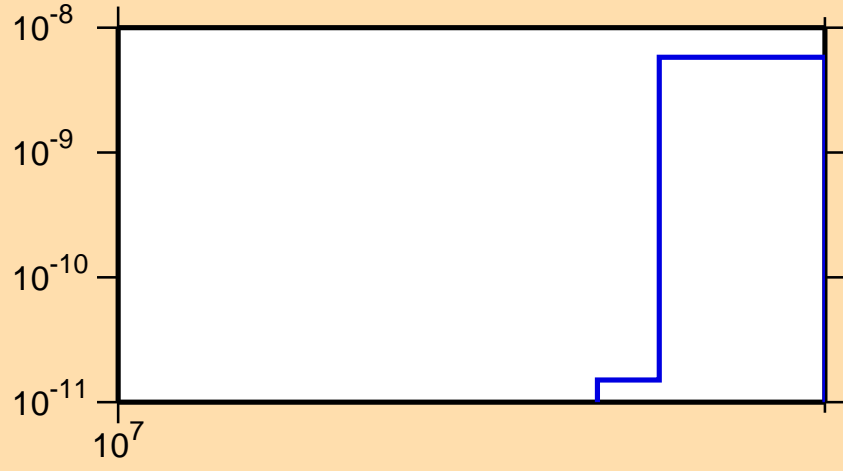
\sigma vs. E for ^{130}\text{Ce}(n,2n\alpha)
