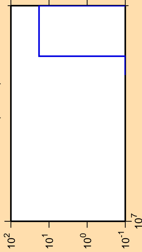
\Delta\sigma/\sigma vs. E for ^{130}\text{Ce} (mt 34)
