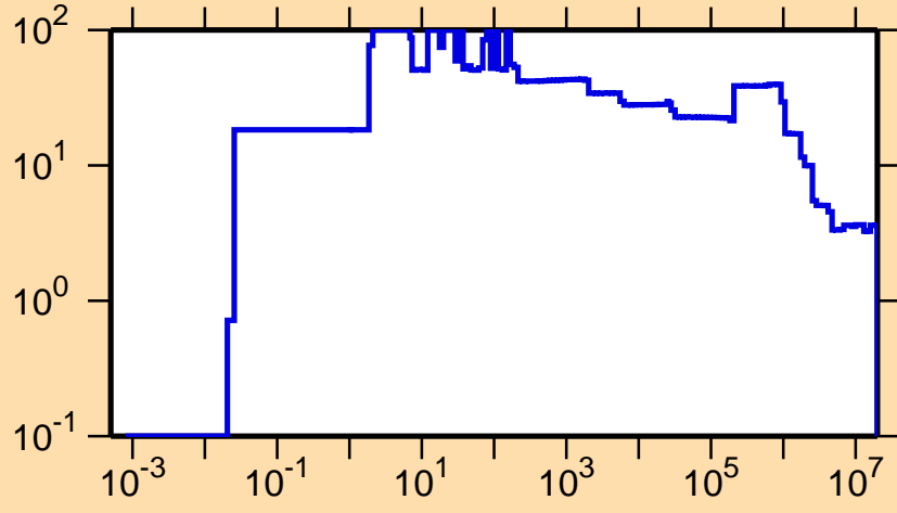
\Delta\sigma/\sigma vs. E for ^{130}\text{Ce}(n,\text{nonel.})
