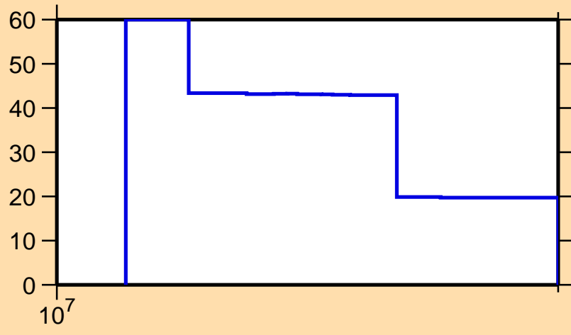
\Delta\sigma/\sigma vs. E for ^{130}\text{Ce}(n,2n)
