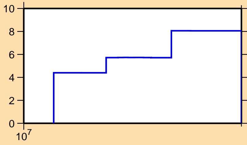
\Delta\sigma/\sigma vs. E for ^{130}\text{Ce}(n,\text{el.})
