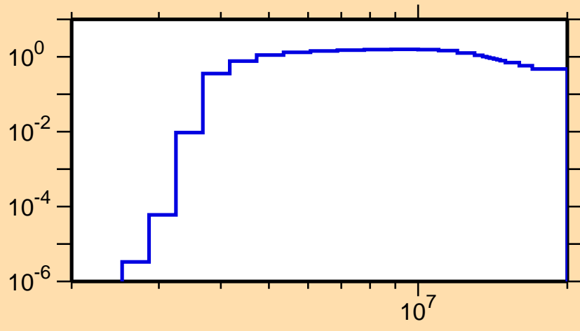
\sigma vs. E for ^{130}\text{Ce}(n,n\text{cont.})
