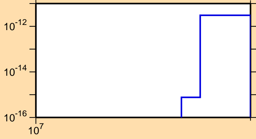
\sigma vs. E for ^{130}\text{Ce} (mt 34)
