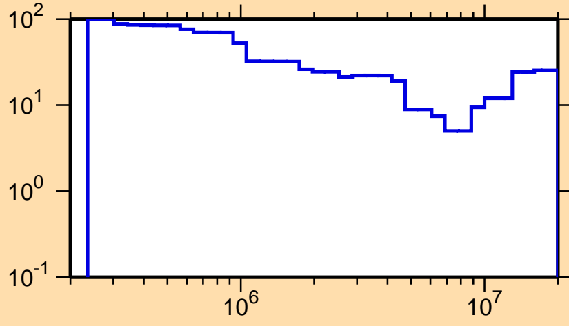
\Delta\sigma/\sigma vs. E for ^{130}\text{Ce}(n,\text{inel.})
