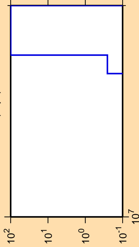
\Delta\sigma/\sigma vs. E for ^{130}\text{Ce}(n,\text{pt})
