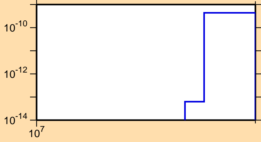
\sigma vs. E for ^{130}\text{Ce}(n,\text{pt})
