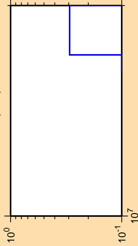
\Delta\sigma/\sigma vs. E for ^{130}\text{Ce}(n,nt)
