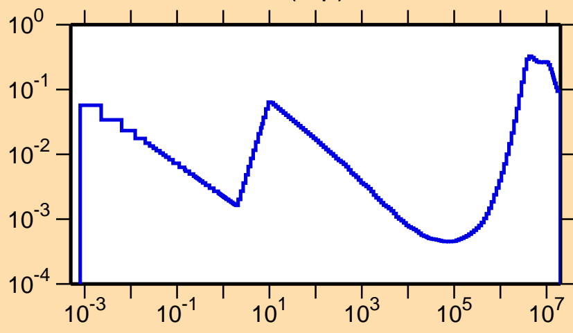
\sigma vs. E for ^{130}\text{Ce}(n,p)
