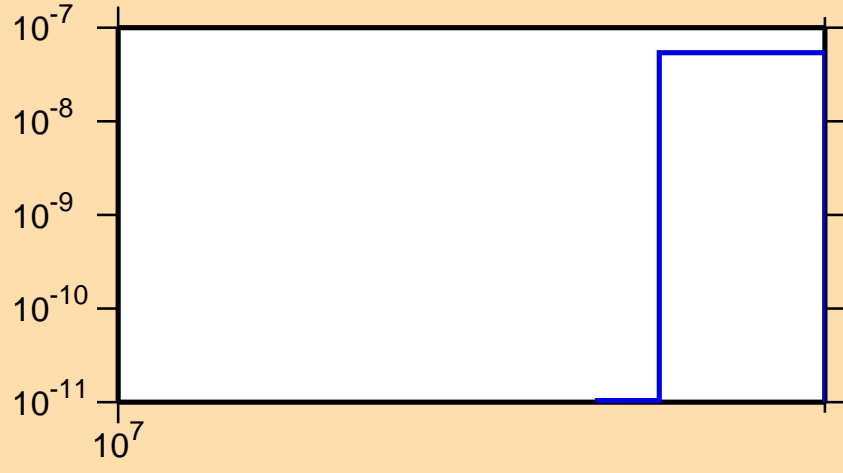
\sigma vs. E for ^{130}\text{Ce}(n,\text{nd})
