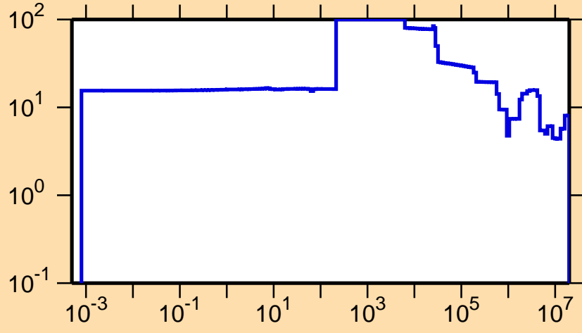
\Delta\sigma/\sigma vs. E for ^{130}\text{Ce}(n,\text{el.})
