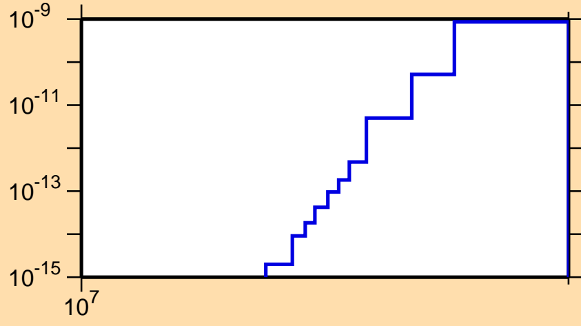
\sigma vs. E for ^{130}\text{Ce}(\text{mt117})
