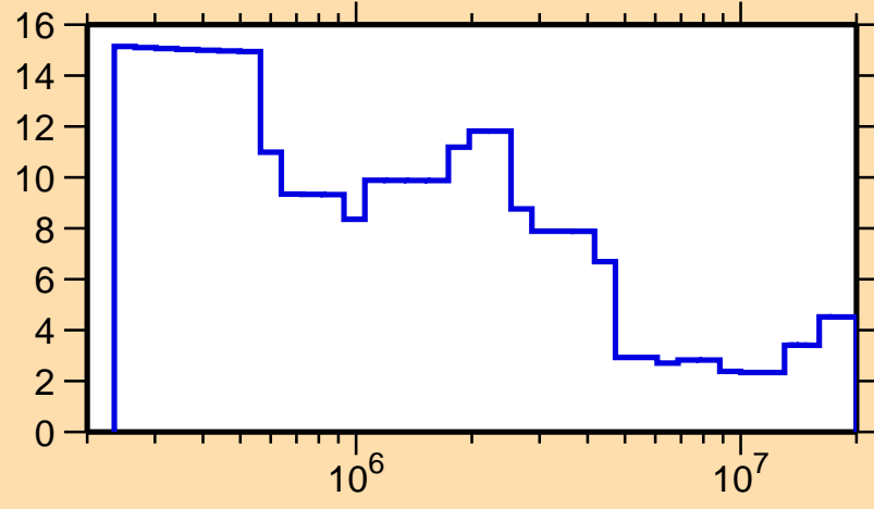
\Delta\sigma/\sigma vs. E for ^{130}\text{Ce}(n,\text{tot.})
