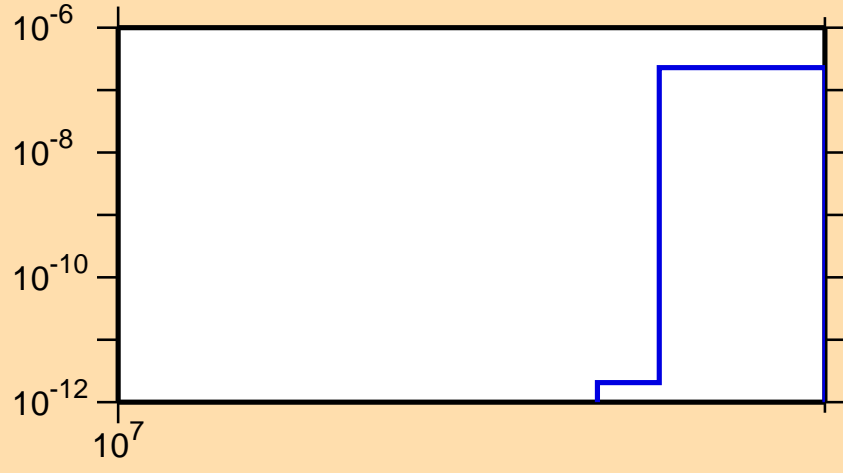
\sigma vs. E for ^{130}\text{Ce}(n,2np)
