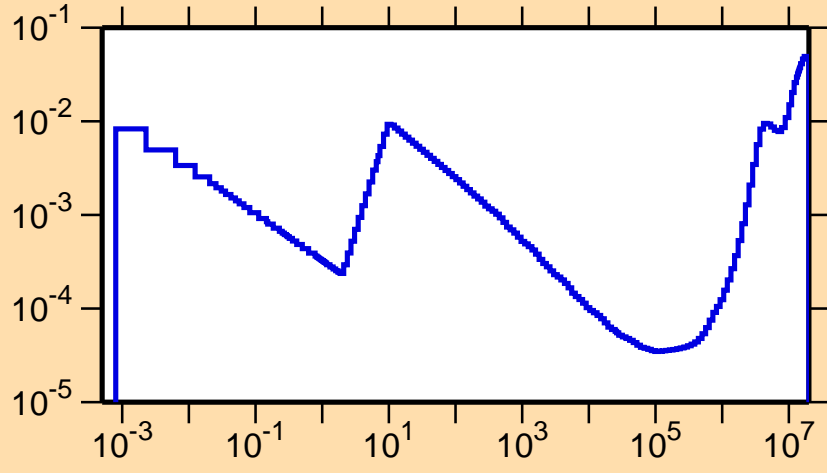
\sigma vs. E for ^{130}\text{Ce}(n,\alpha)
