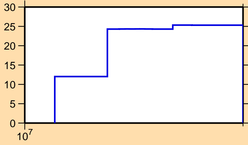
\Delta\sigma/\sigma vs. E for ^{130}\text{Ce}(n,\text{inel.})
