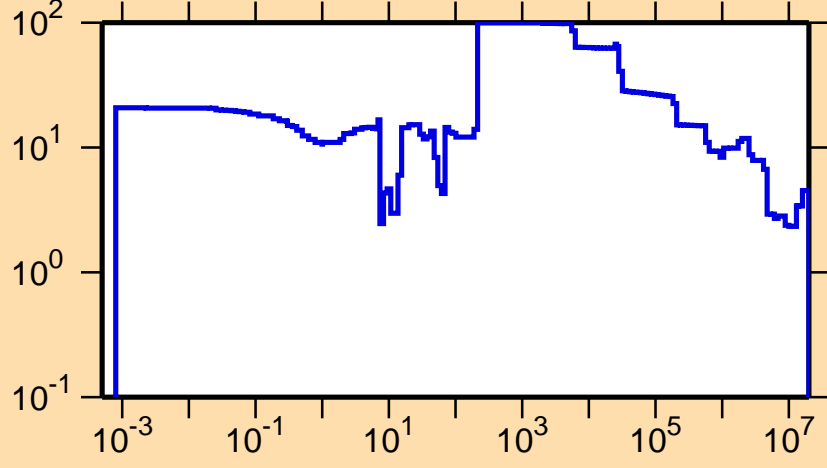
\Delta\sigma/\sigma vs. E for ^{130}\text{Ce}(n,\text{tot.})
