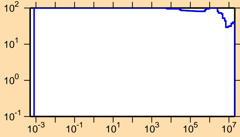
\Delta\sigma/\sigma vs. E for ^{130}\text{Ce}(n,p)
