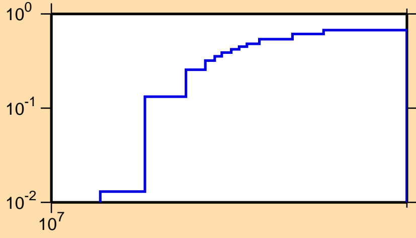
\sigma vs. E for ^{130}\text{Ce}(n,2n)
