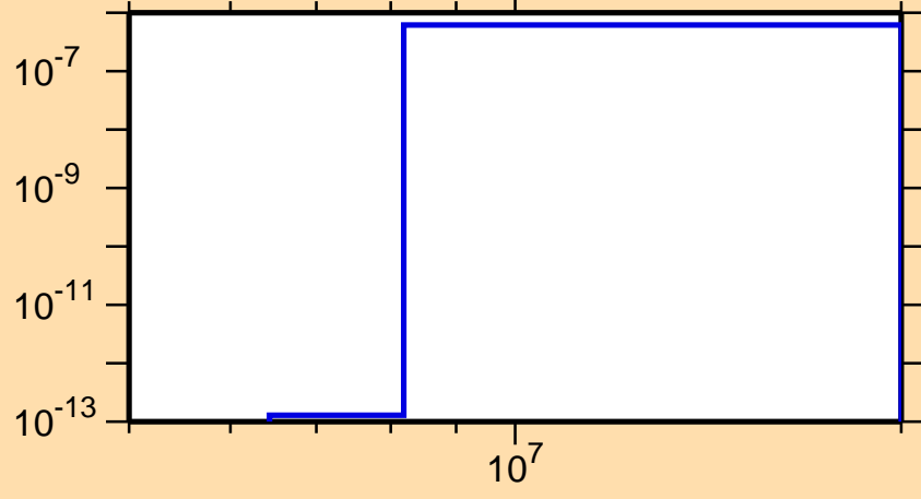
\sigma vs. E for ^{130}\text{Ce}(n,\text{He3})
