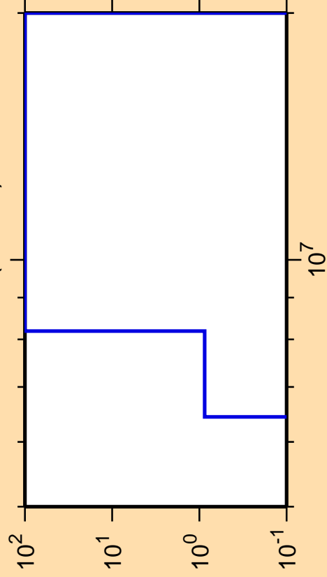
\Delta\sigma/\sigma vs. E for ^{130}\text{Ce}(n,\text{He3})
