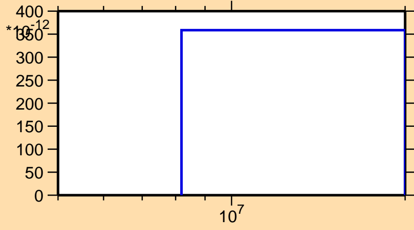
\sigma vs. E for ^{130}\text{Ce}(\text{mt } 45)
