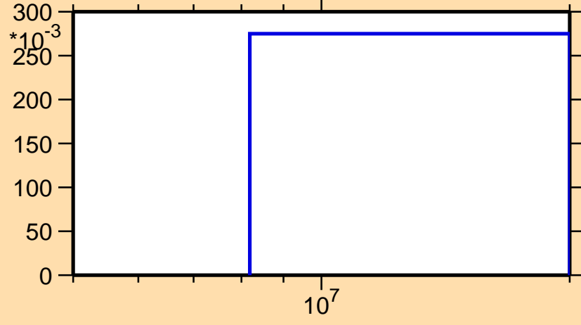
\sigma vs. E for ^{130}\text{Ce}(n,2n)
