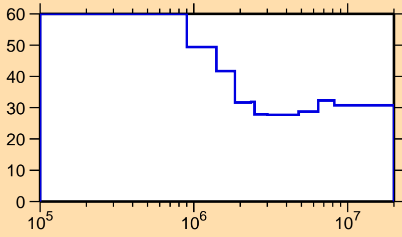
\Delta\sigma/\sigma vs. E for ^{130}\text{Ce}(n,n_1)
