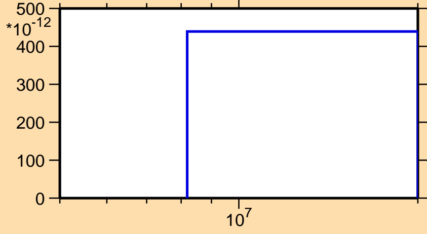
\sigma vs. E for ^{130}\text{Ce}(n,\text{nd})
