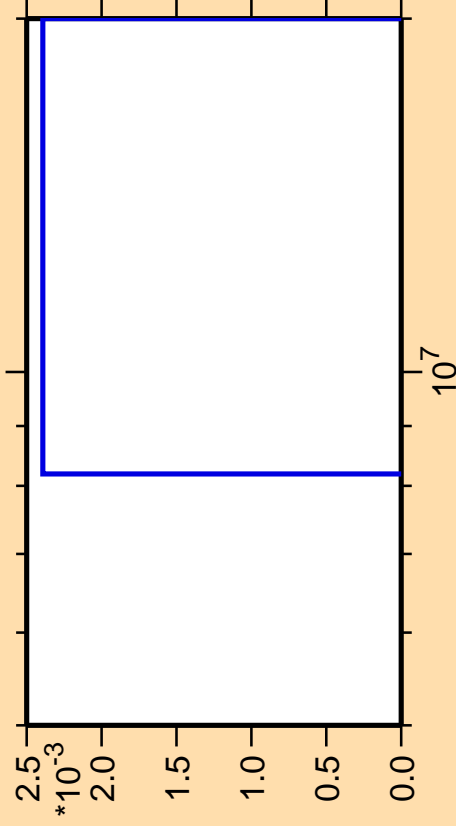
\Delta\sigma/\sigma vs. E for ^{130}\text{Ce}(n,nt)
