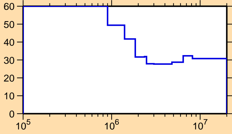
\Delta\sigma/\sigma vs. E for ^{130}\text{Ce}(n,n_1)
