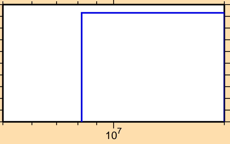
\sigma vs. E for ^{130}\text{Ce}(n,2np)
