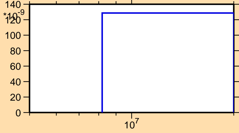
\sigma vs. E for ^{130}\text{Ce}(n,\text{pd})
