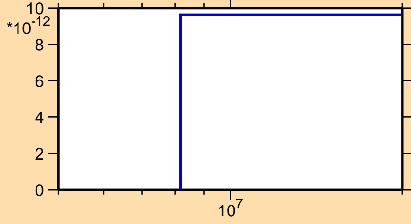
\sigma vs. E for ^{130}\text{Ce}(\text{mt117})
