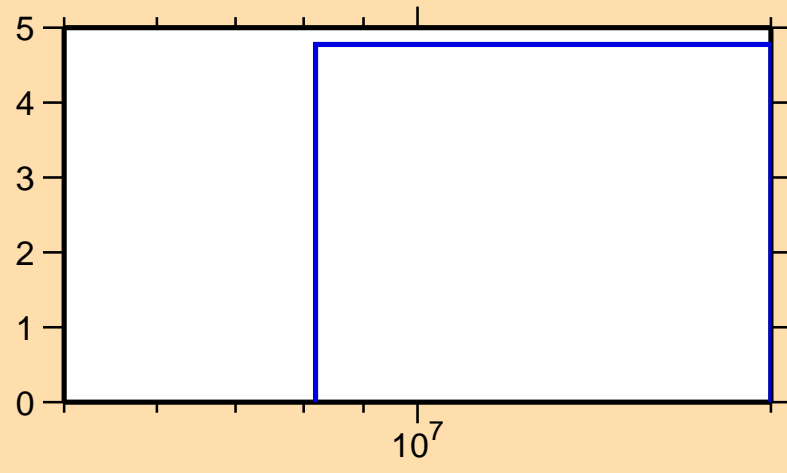
\Delta\sigma/\sigma vs. E for ^{130}\text{Ce}(n,\text{el.})
