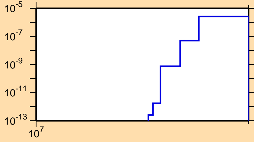
\sigma vs. E for ^{135}\text{Ce}(n,\text{nd})
