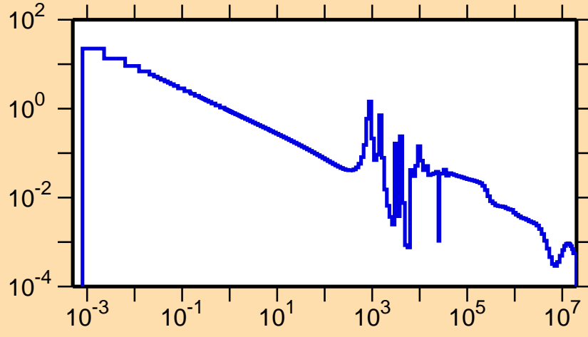
\sigma vs. E for ^{146}\text{Ce}(n,\gamma)
