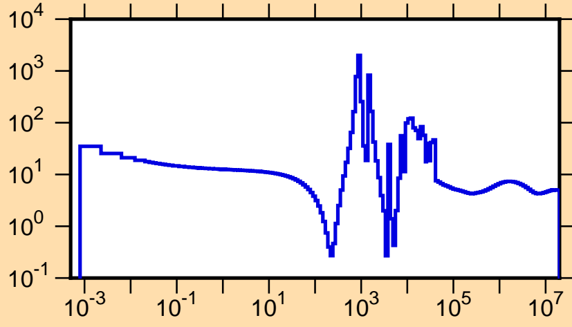
\sigma vs. E for ^{146}\text{Ce}(n,\text{tot.})
