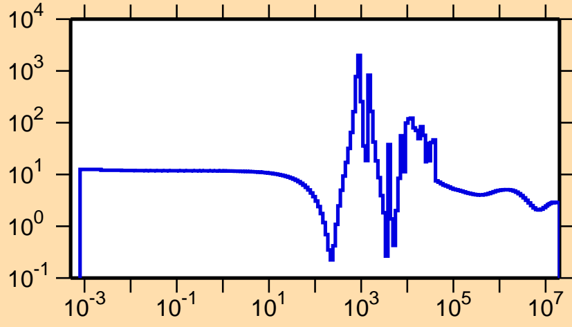
\sigma vs. E for ^{146}\text{Ce}(n,\text{el.})
