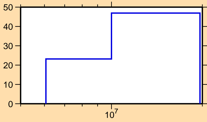
\Delta\sigma/\sigma vs. E for ^{146}\text{Ce}(n,ncont.)
