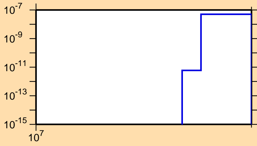
\sigma vs. E for ^{147}\text{Ce}(n,2np)
