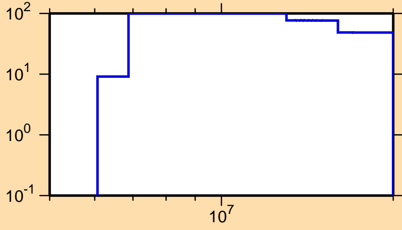
\Delta\sigma/\sigma vs. E for ^{147}\text{Ce}(n,p)
