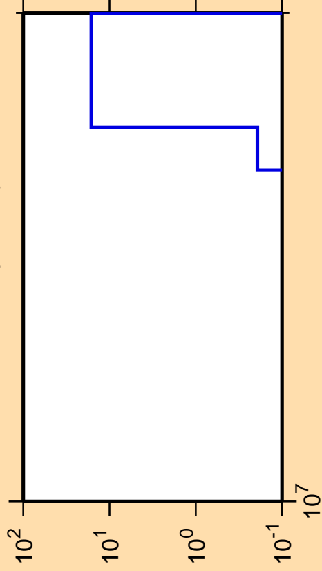
\Delta\sigma/\sigma vs. E for ^{147}\text{Ce}(n,3n\alpha)
