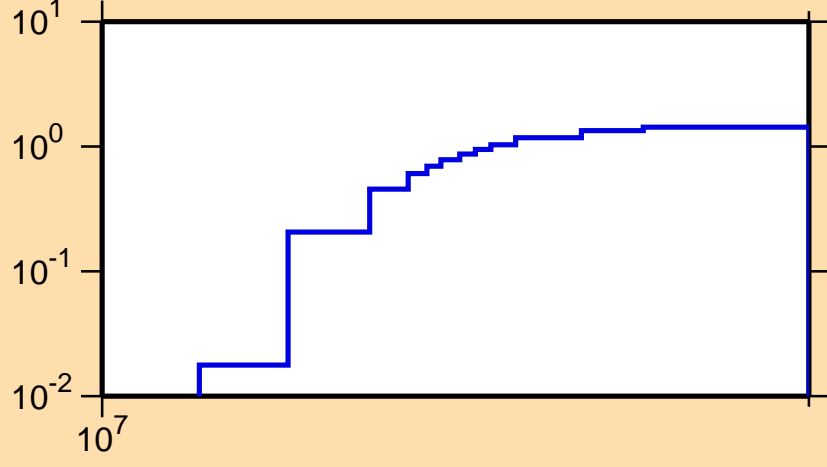
\sigma vs. E for ^{147}\text{Ce}(n,3n)
