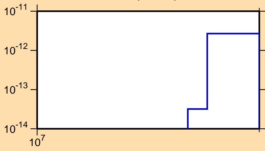
\sigma vs. E for ^{147}\text{Ce}(n,3n\alpha)
