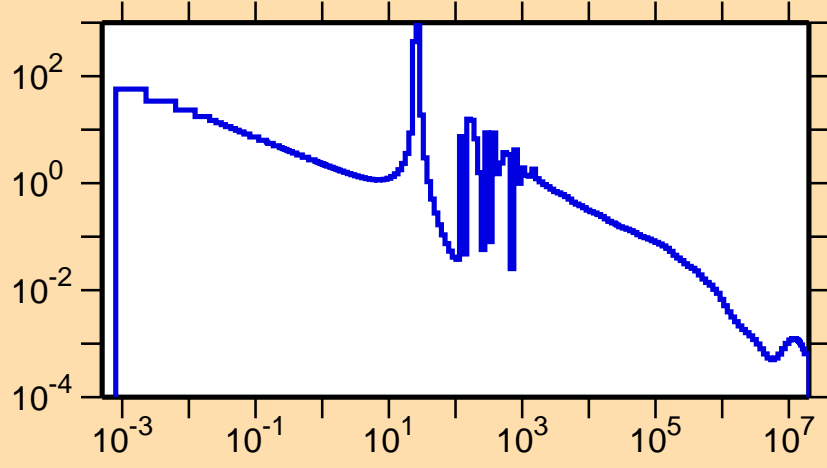
\sigma vs. E for ^{147}\text{Ce}(n,\gamma)
