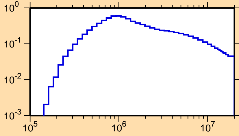
\sigma vs. E for ^{250}\text{Cf}(n,n_2)
