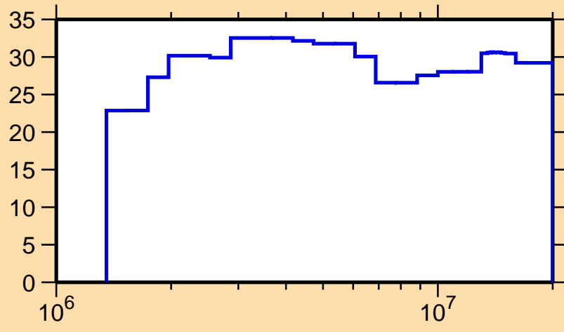
\Delta\sigma/\sigma vs. E for ^{250}\text{Cf}(n,n_1)
