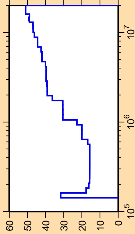
\Delta\sigma/\sigma vs. E for ^{250}\text{Cf}(n,n_2)
