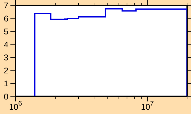
\Delta\sigma/\sigma vs. E for ^{250}\text{Cf}(n,n\text{oncl.})
