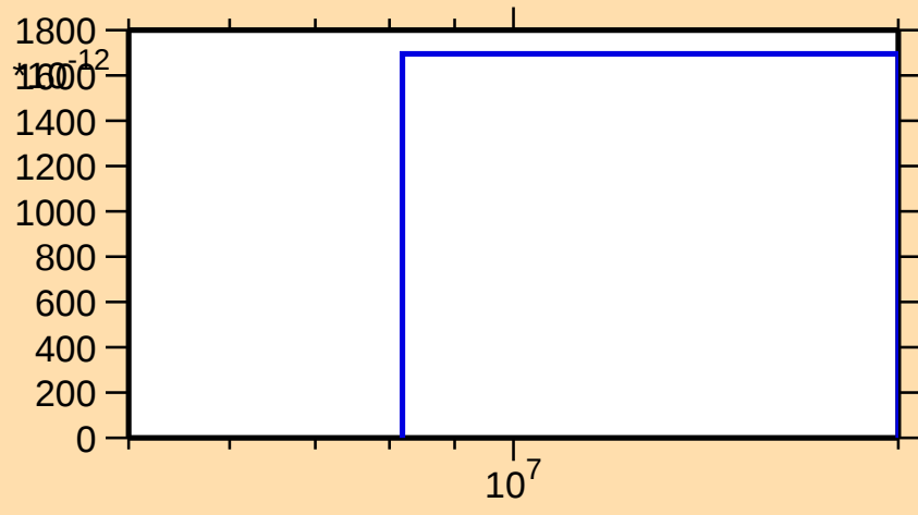
\sigma vs. E for ^{250}\text{Cf}(n,2n\alpha)
