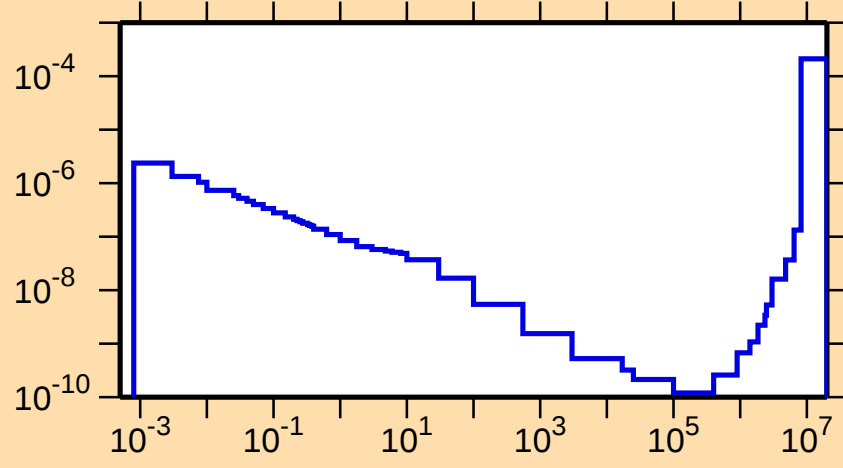
\sigma vs. E for ^{250}\text{Cf}(n,\alpha)
