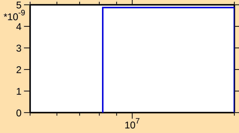
\sigma vs. E for ^{250}\text{Cf}(n,nt)
