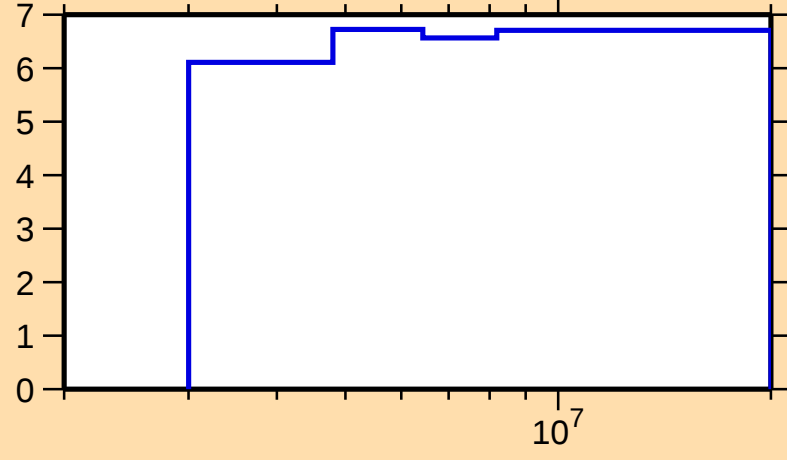
\Delta\sigma/\sigma vs. E for ^{250}\text{Cf}(n,\text{nonel.})
