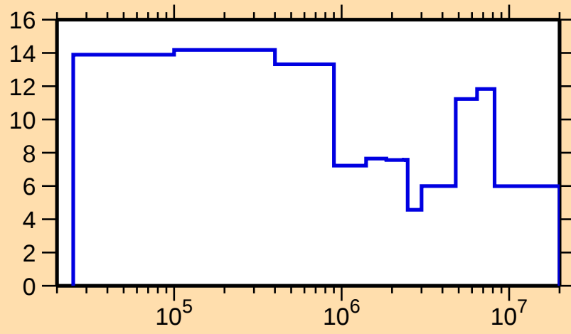
\Delta\sigma/\sigma vs. E for ^{250}\text{Cf}(n,\text{el.})
