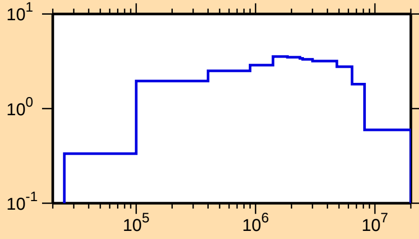
\sigma vs. E for ^{250}\text{Cf}(n,\text{inel.})
