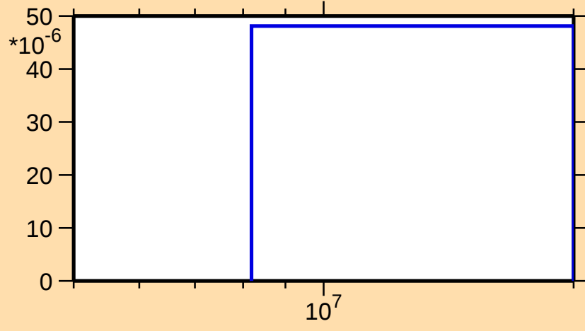
\sigma vs. E for ^{250}\text{Cf}(n,d)
