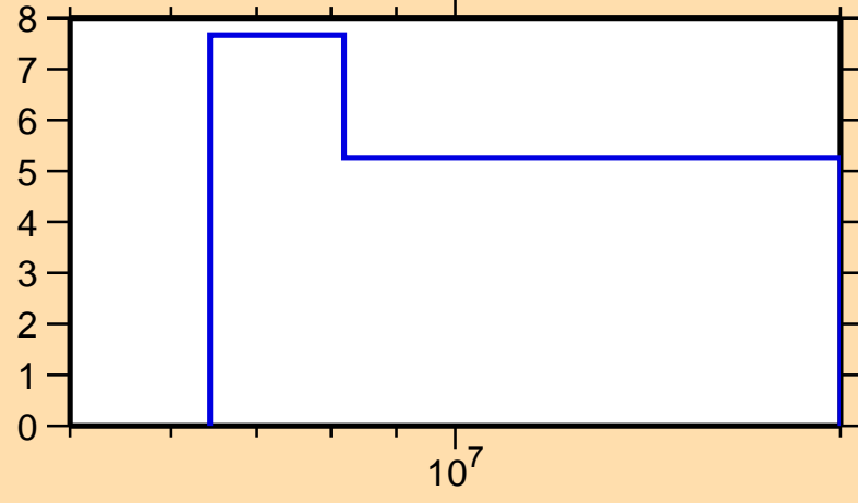
\Delta\sigma/\sigma vs. E for ^{256}\text{Cf}(n,\text{tot.})
