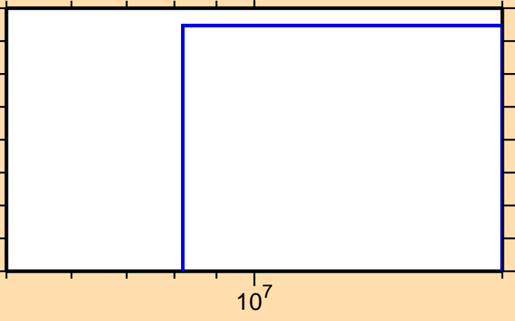
\sigma vs. E for ^{256}\text{Cf}(n,np)
