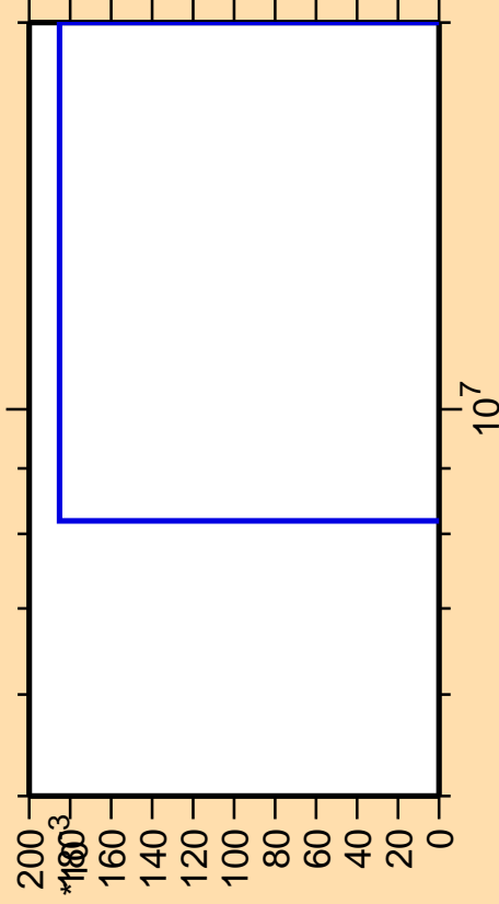
\Delta\sigma/\sigma vs. E for ^{256}\text{Cf}(n,3n\alpha)
