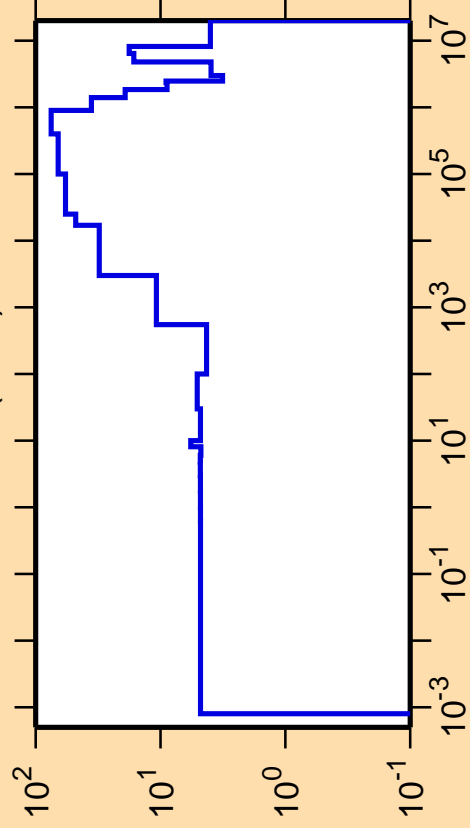
\Delta\sigma/\sigma vs. E for ^{256}\text{Cf}(n,\text{el.})
