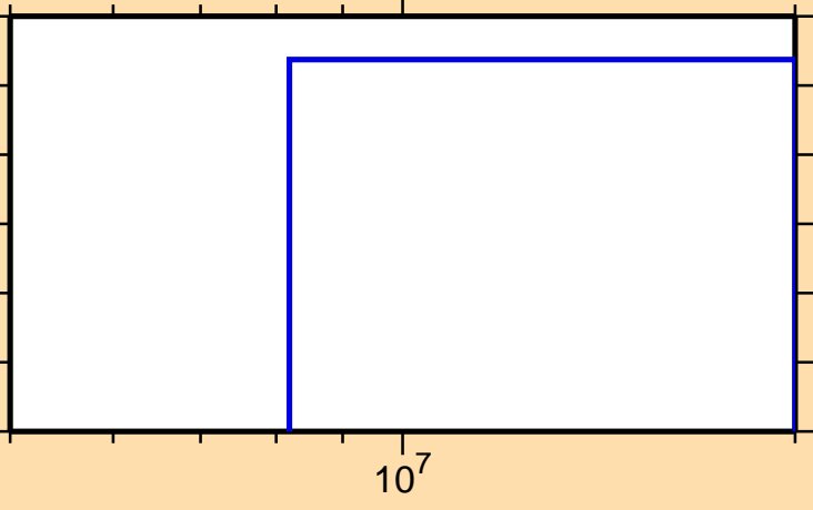
\sigma vs. E for ^{256}\text{Cf}(n,d)
