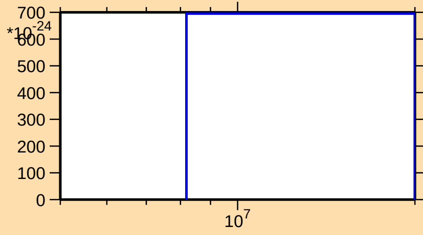
\sigma vs. E for ^{38}\text{Cl}(\text{mt } 45)
