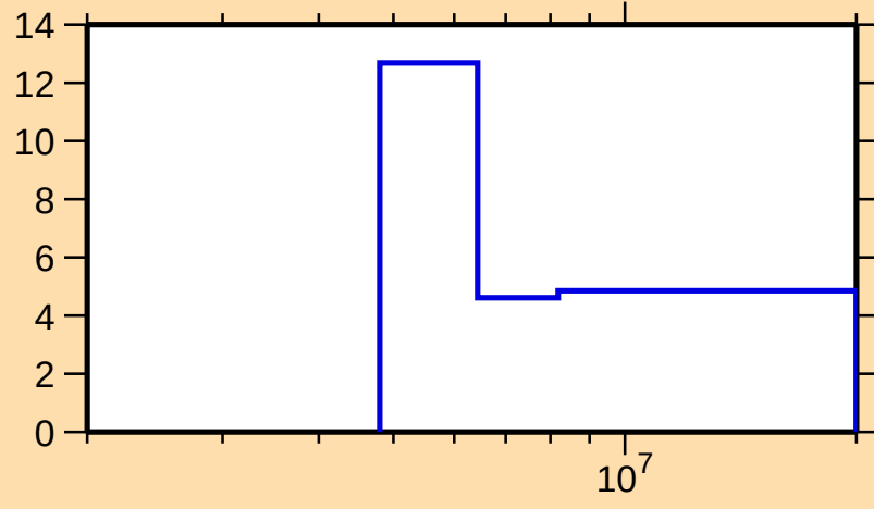
\Delta\sigma/\sigma vs. E for ^{38}\text{Cl}(n,2n)
