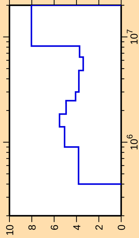
\Delta\sigma/\sigma vs. E for ^{38}\text{Cl}(n,\text{inel.})
