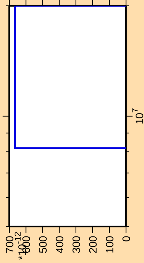
\Delta\sigma/\sigma vs. E for ^{38}\text{Cl}(\text{mt } 45)
