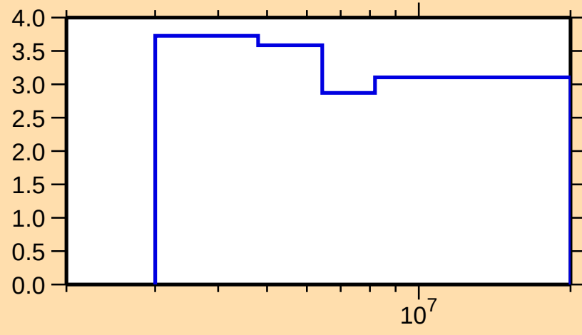
\Delta\sigma/\sigma vs. E for ^{38}\text{Cl}(n,n\text{oncl.})
