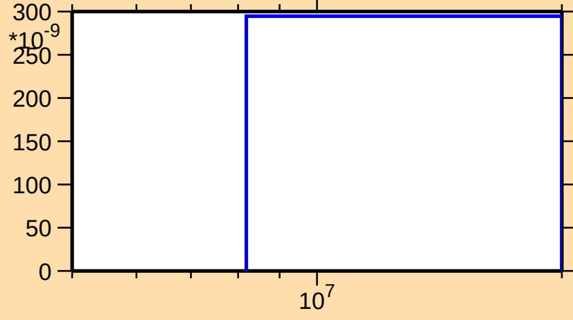
\sigma vs. E for ^{38}\text{Cl}(n,2n\alpha)
