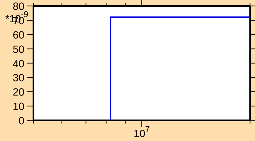
\sigma vs. E for ^{38}\text{Cl}(n,\text{nt})
