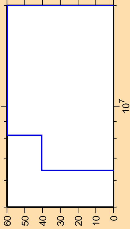
\Delta\sigma/\sigma vs. E for ^{65}\text{Co}(n,p)
