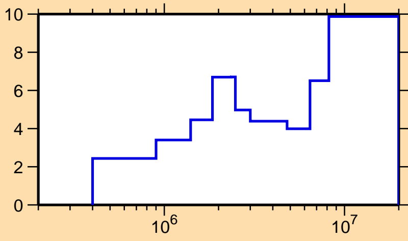
\Delta\sigma/\sigma vs. E for ^{65}\text{Co}(n,\text{el.})
