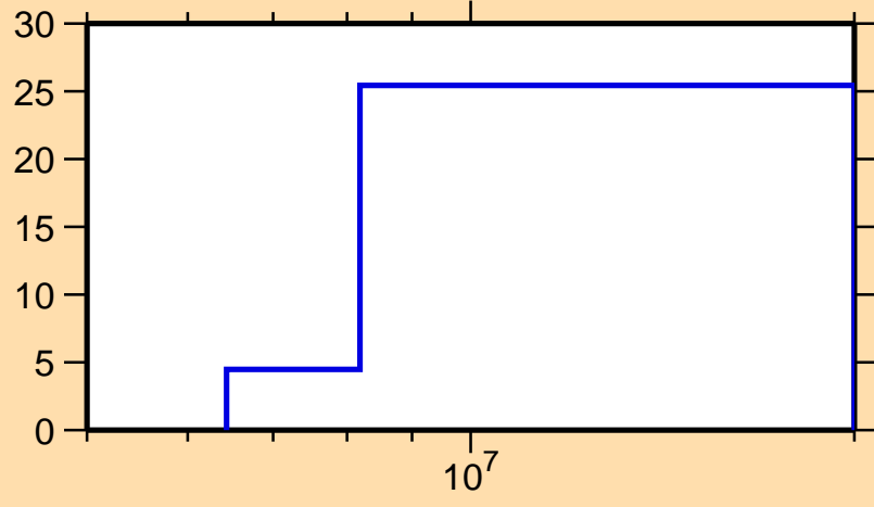
\Delta\sigma/\sigma vs. E for ^{65}\text{Co}(n,ncont.)
