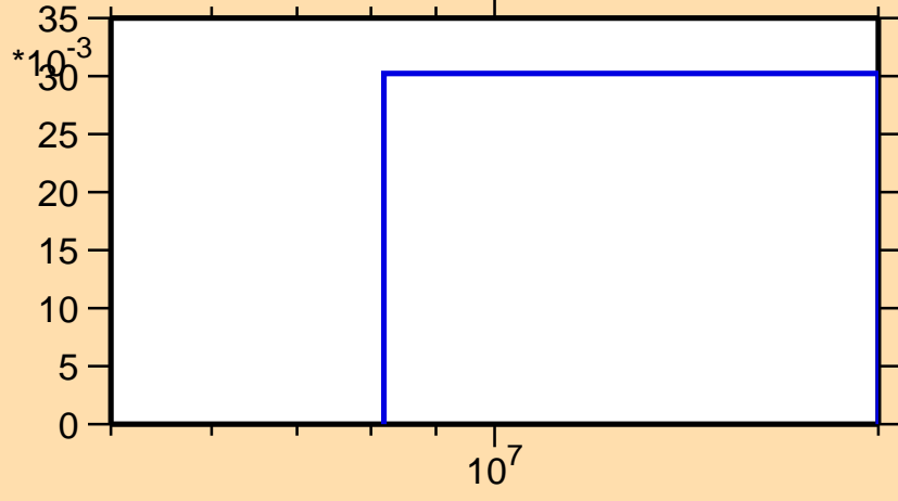
\sigma vs. E for ^{65}\text{Co}(n,3n)
