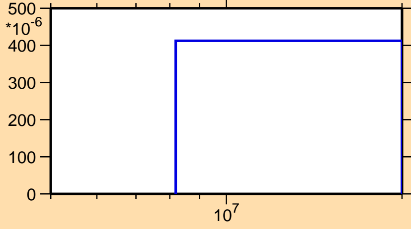
\sigma vs. E for ^{65}\text{Co}(n,d)
