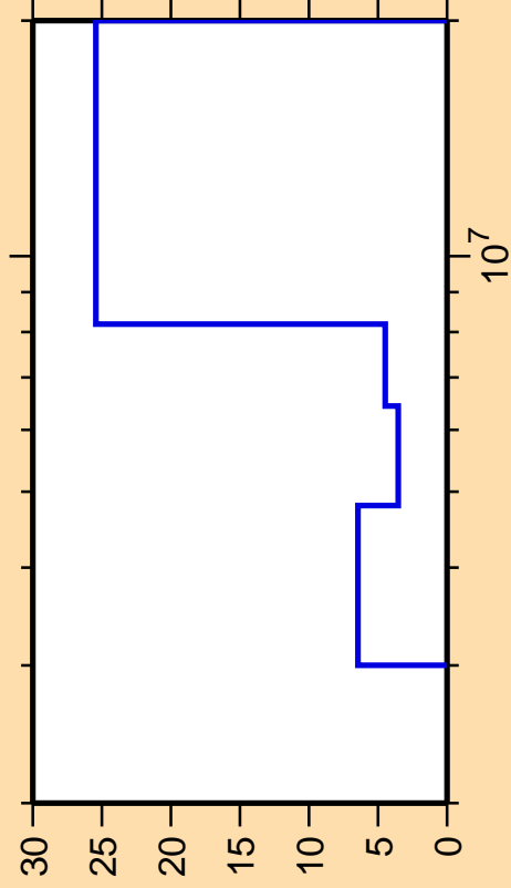
\Delta\sigma/\sigma vs. E for ^{65}\text{Co}(n,n\text{cont.})
