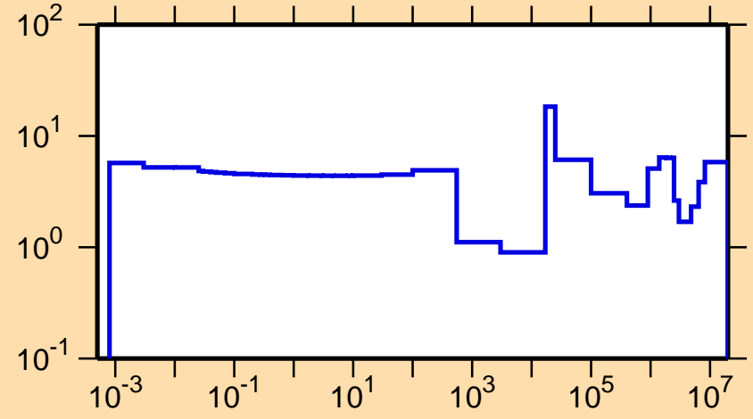
\Delta\sigma/\sigma vs. E for ^{65}\text{Co}(n,\text{tot.})
