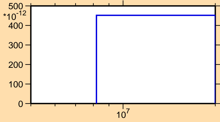
\sigma vs. E for ^{65}\text{Co}(n,\text{nd})
