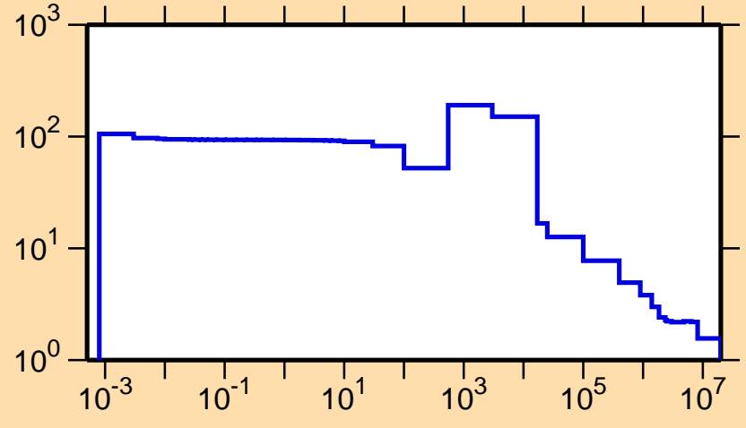
\sigma vs. E for ^{65}\text{Co}(n,\text{el.})
