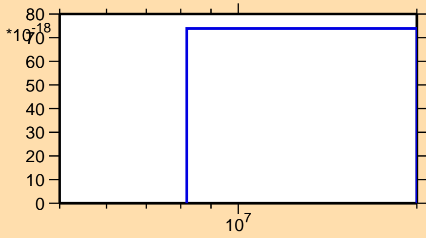
\sigma vs. E for ^{65}\text{Co}(n,2np)
