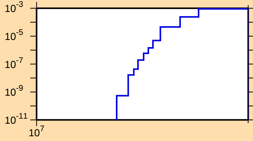
\sigma vs. E for ^{64}\text{Cu}(n,\text{nd})
