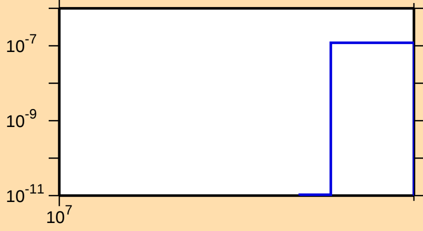
\sigma vs. E for ^{64}\text{Cu}(n,\text{nt})
