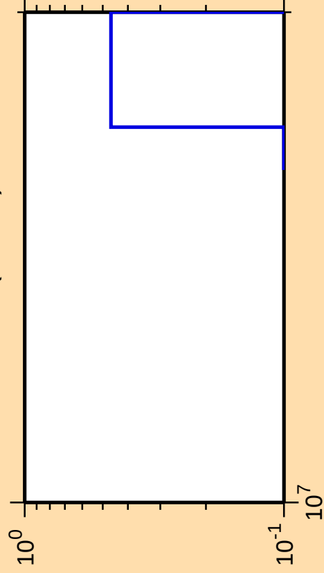
\Delta\sigma/\sigma vs. E for ^{64}\text{Cu}(\text{mt117})
