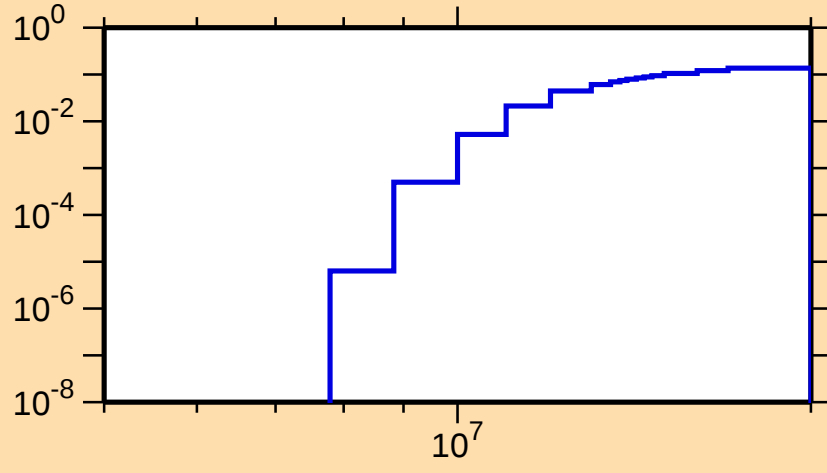
\sigma vs. E for ^{64}\text{Cu}(n,np)
