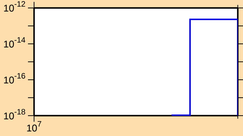
\sigma vs. E for ^{64}\text{Cu}(\text{mt117})
