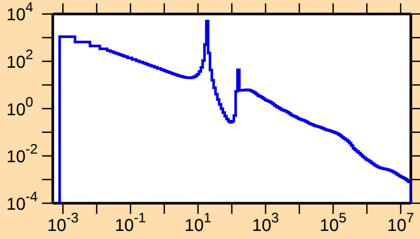
\sigma vs. E for ^{64}\text{Cu}(n,\gamma)
