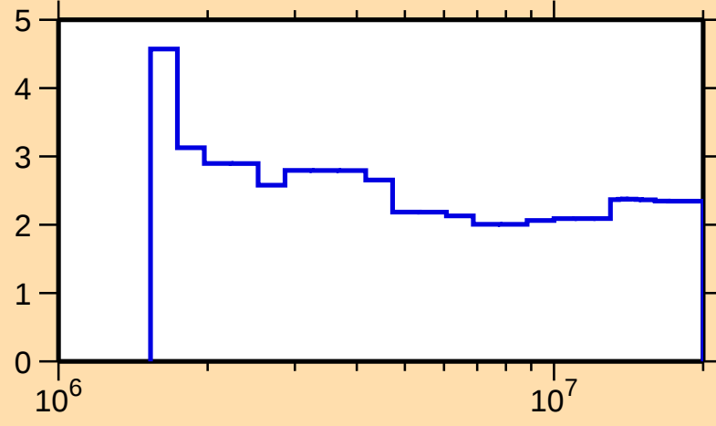
\Delta\sigma/\sigma vs. E for ^{64}\text{Cu}(n,n\text{oncl.})
