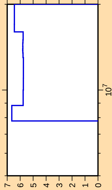
\Delta\sigma/\sigma vs. E for ^{64}\text{Cu}(n,2n)
