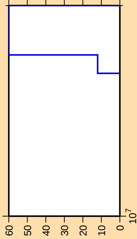
\Delta\sigma/\sigma vs. E for ^{64}\text{Cu}(n,\text{nt})
