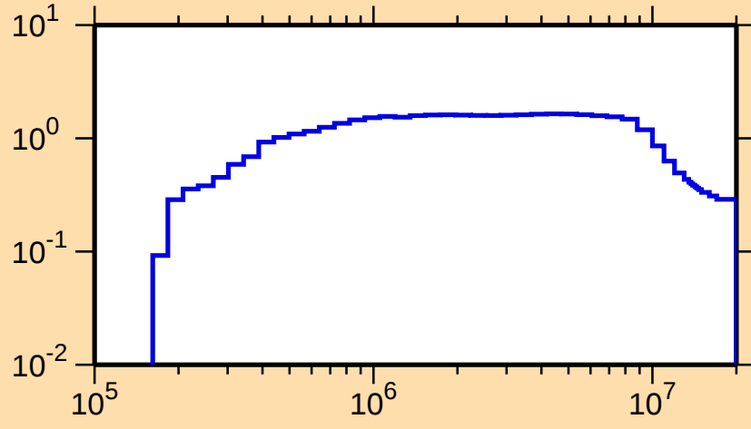
\sigma vs. E for ^{64}\text{Cu}(n,\text{inel.})
