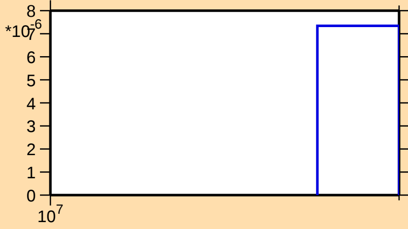
\sigma vs. E for ^{64}\text{Cu}(n,3n)
