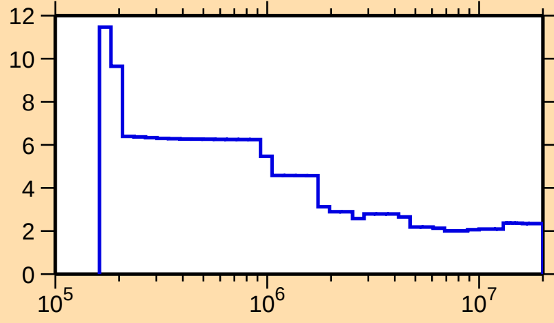
\Delta\sigma/\sigma vs. E for ^{64}\text{Cu}(\text{n,nonel.})
