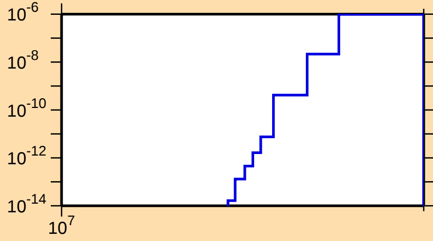
\sigma vs. E for ^{64}\text{Cu}(n,\text{He3})
