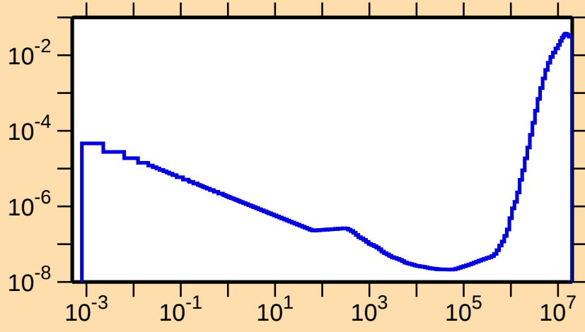
\sigma vs. E for ^{64}\text{Cu}(n,\alpha)
