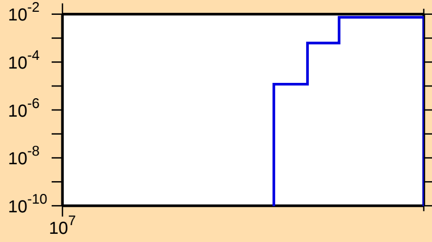
\sigma vs. E for ^{64}\text{Cu}(n,2np)
