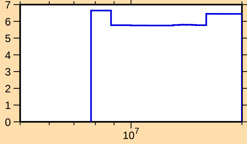
\Delta\sigma/\sigma vs. E for ^{64}\text{Cu}(n,2n)
