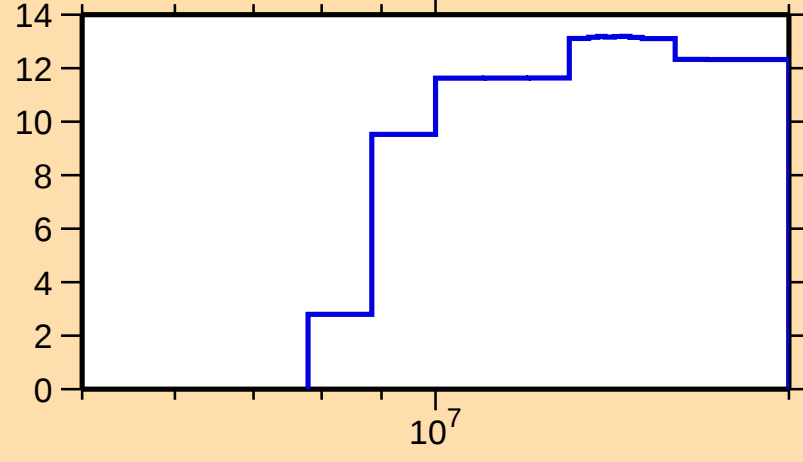
\Delta\sigma/\sigma vs. E for ^{64}\text{Cu}(n,\text{inel.})
