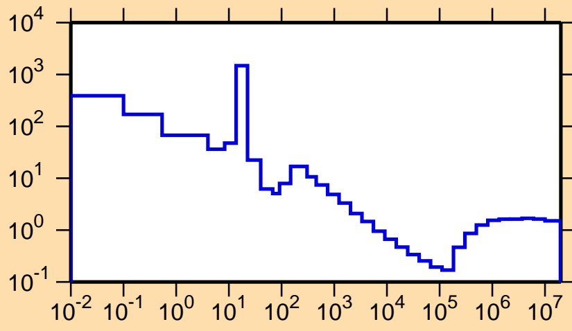
\sigma vs. E for ^{64}\text{Cu}(n,\text{nonel.})
