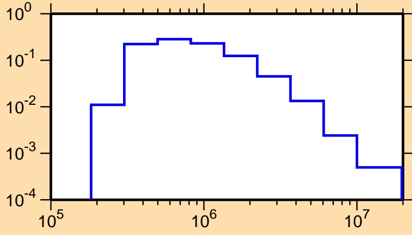
\sigma vs. E for ^{64}\text{Cu}(n,n_2)
