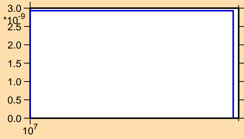
\sigma vs. E for ^{74}\text{Cu}(n,nt)
