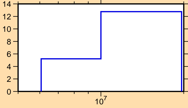
\Delta\sigma/\sigma vs. E for ^{74}\text{Cu}(n,el.)
