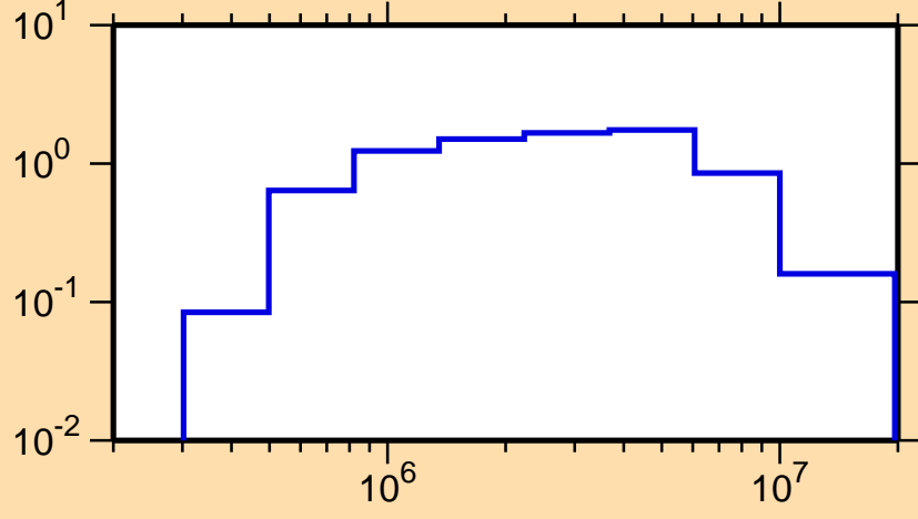
\sigma vs. E for ^{74}\text{Cu}(n,\text{inel.})
