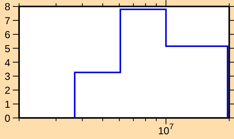
\Delta\sigma/\sigma vs. E for ^{264}
