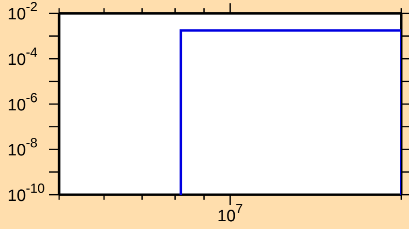
\sigma vs. E for ^{155}\text{Dy}(n,np)
