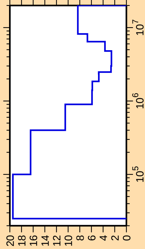
\Delta\sigma/\sigma vs. E for ^{155}\text{Dy}(n,\text{inel.})
