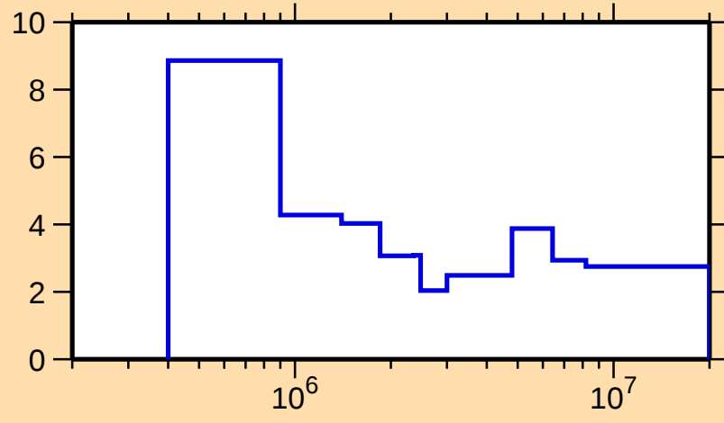
\Delta\sigma/\sigma vs. E for ^{155}\text{Dy}(n,\text{nonel.})
