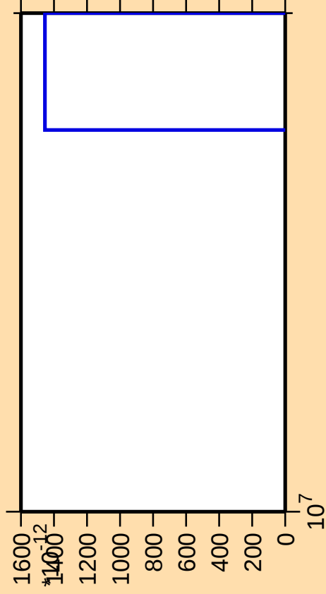
\Delta\sigma/\sigma vs. E for ^{167}\text{Dy} (mt 11)
