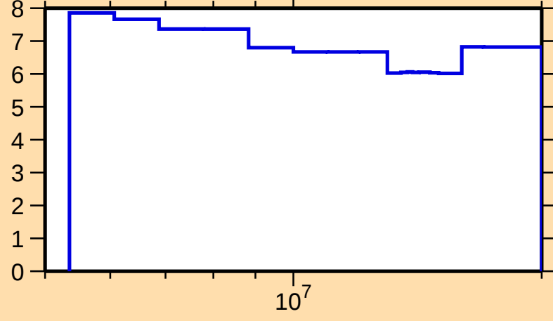
\Delta\sigma/\sigma vs. E for ^{167}\text{Dy}(n,\text{nonel.})
