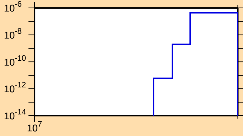
\sigma vs. E for ^{167}\text{Dy}(n,nd)
