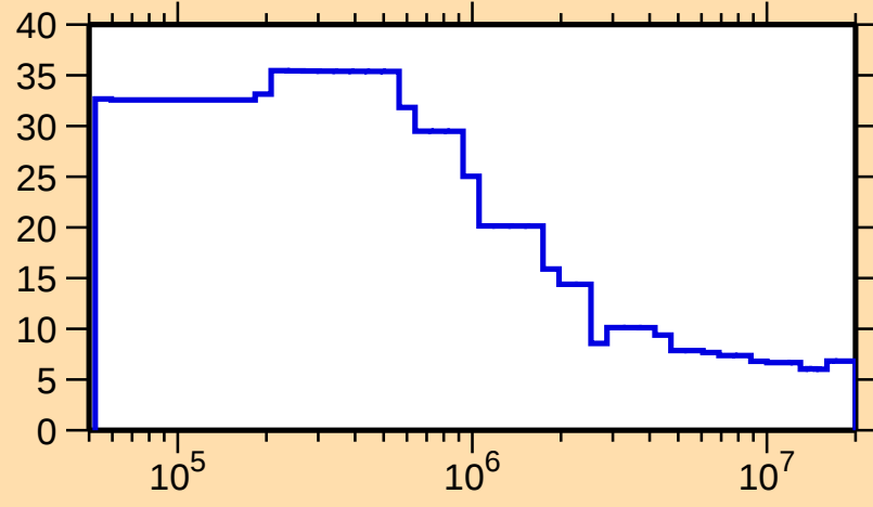
\Delta\sigma/\sigma vs. E for ^{167}\text{Dy}(n,\text{nonel.})
