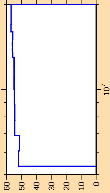
\Delta\sigma/\sigma vs. E for ^{167}\text{Dy}(n,\gamma)
