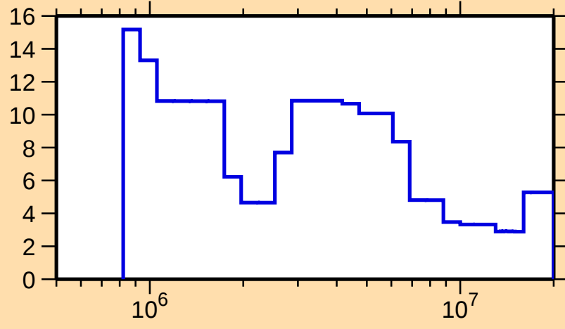
\Delta\sigma/\sigma vs. E for ^{167}\text{Dy}(n, tot.)
