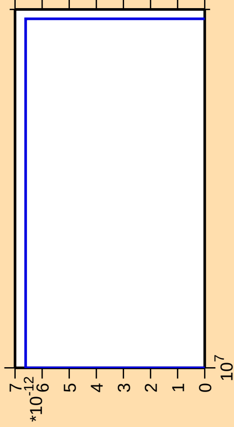
\Delta\sigma/\sigma vs. E for ^{167}\text{Dy}(\text{mt } 11)
