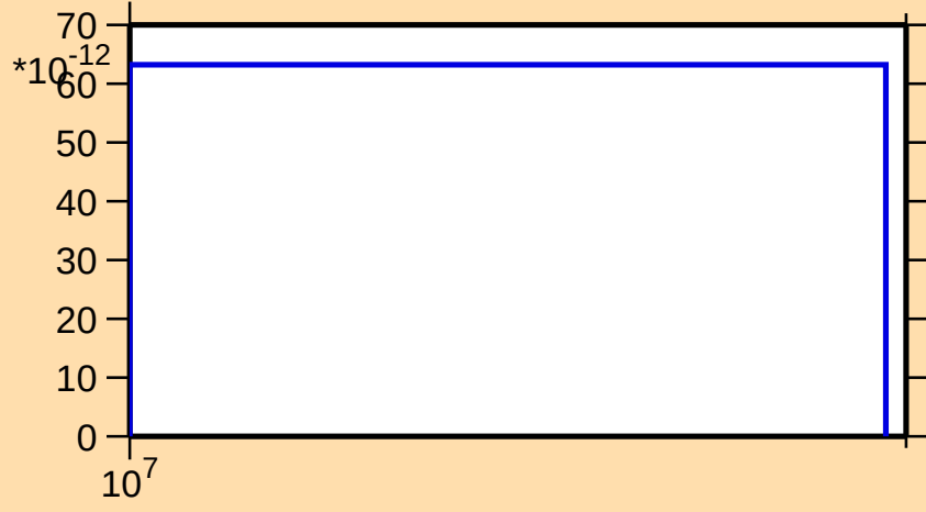
\sigma vs. E for ^{167}\text{Dy}(n,2np)
