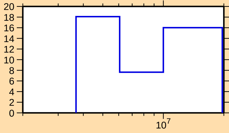
\Delta\sigma/\sigma vs. E for ^{167}\text{Dy}(n,2n)
