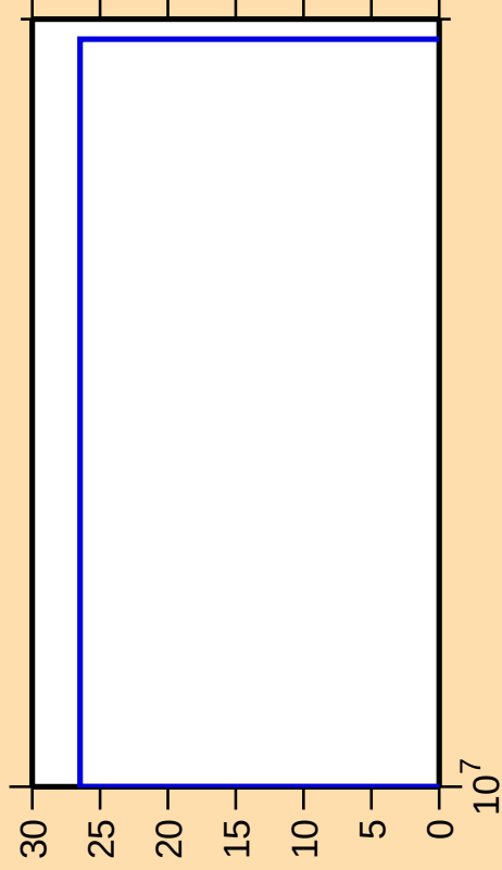
\Delta\sigma/\sigma vs. E for ^{167}\text{Dy}(n,2np)
