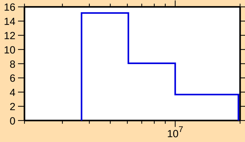
\Delta\sigma/\sigma vs. E for ^{167}\text{Dy}(n,\text{el.})
