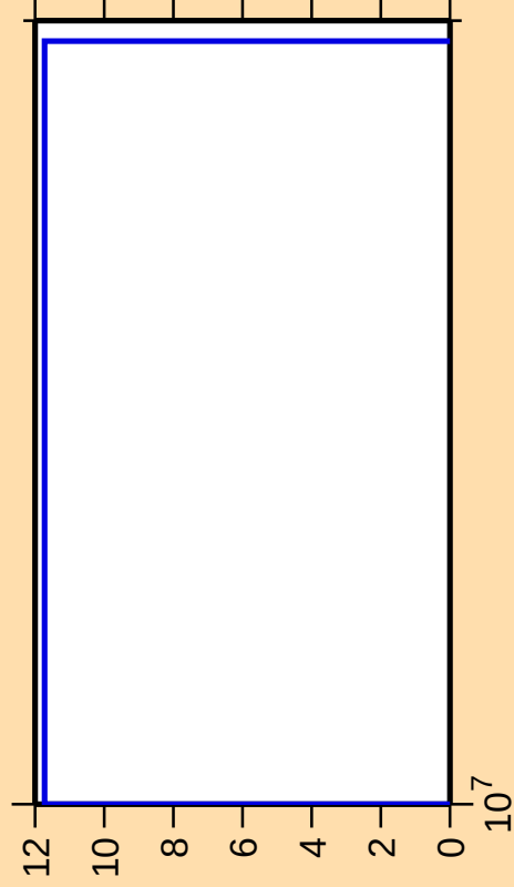
\Delta\sigma/\sigma vs. E for ^{167}\text{Dy}(n,3n)
