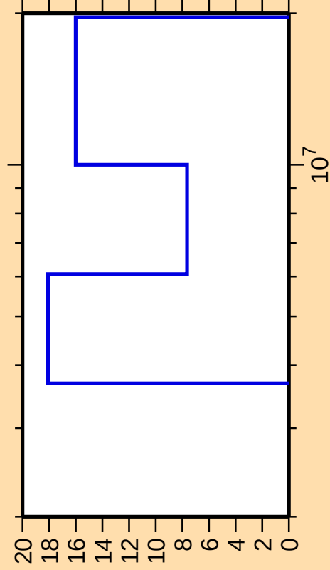
\Delta\sigma/\sigma vs. E for ^{167}\text{Dy}(n,2n)
