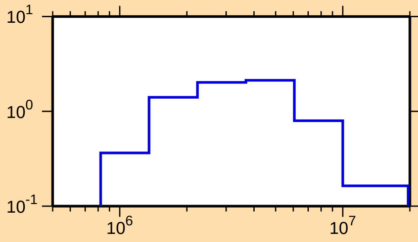
\sigma vs. E for ^{167}\text{Dy}(n,n\text{cont.})
