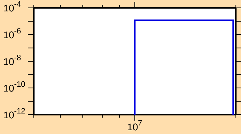
\sigma vs. E for ^{167}\text{Dy}(n,np)
