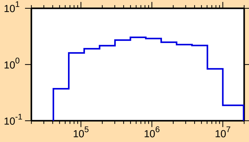
\sigma vs. E for ^{167}\text{Dy}(n,\text{inel.})
