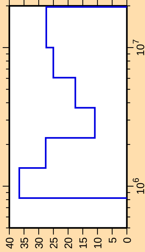
\Delta\sigma/\sigma vs. E for ^{167}\text{Dy}(n,n\text{cont.})
