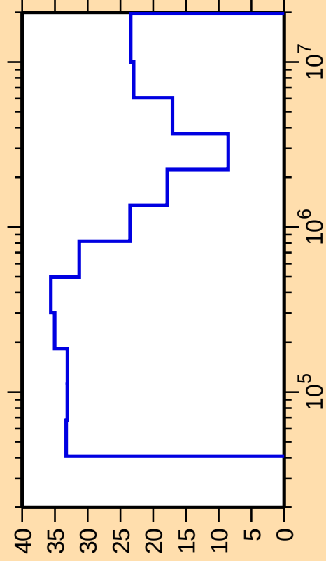
\Delta\sigma/\sigma vs. E for ^{167}\text{Dy}(n,\text{inel.})
