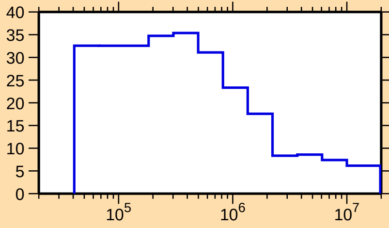
\Delta\sigma/\sigma vs. E for ^{167}\text{Dy}(n,\text{nonel.})
