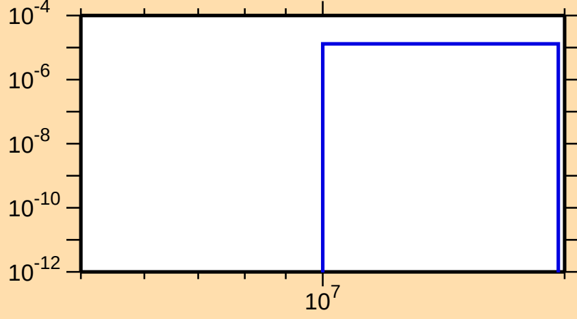
\sigma vs. E for ^{167}\text{Dy}(n,t)
