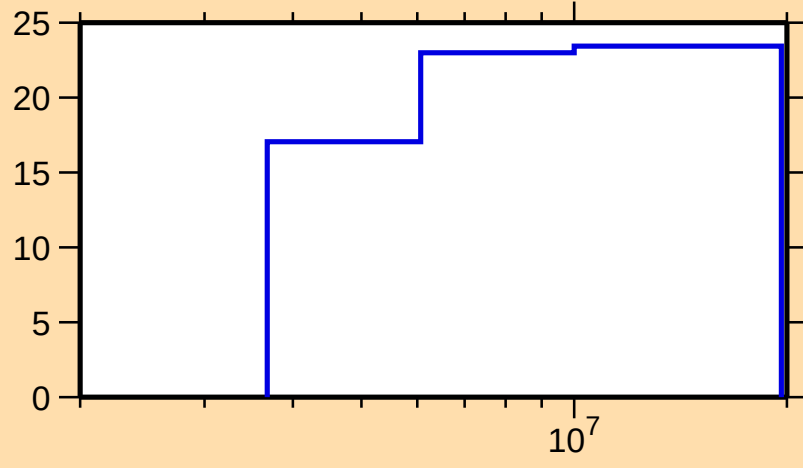
\Delta\sigma/\sigma vs. E for ^{167}\text{Dy}(n,\text{inel.})
