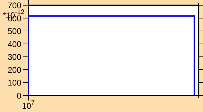
\sigma vs. E for ^{167}\text{Dy}(n,nt)
