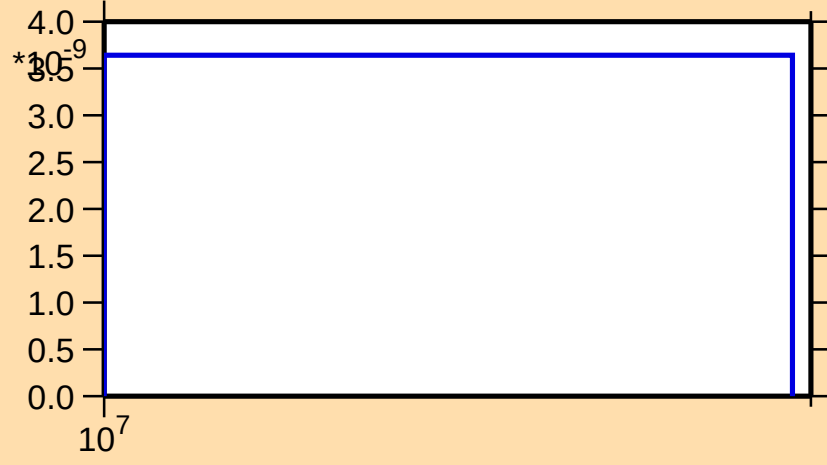
\sigma vs. E for ^{167}\text{Dy}(n,\text{nd})
