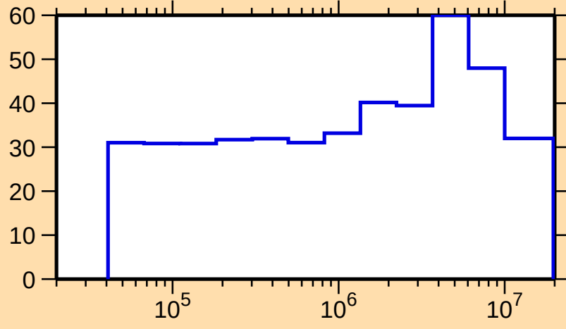
\Delta\sigma/\sigma vs. E for ^{167}\text{Dy}(n,n_1)
