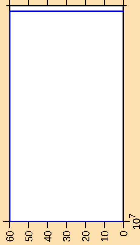
\Delta\sigma/\sigma vs. E for ^{167}\text{Dy}(n,\text{nd})
