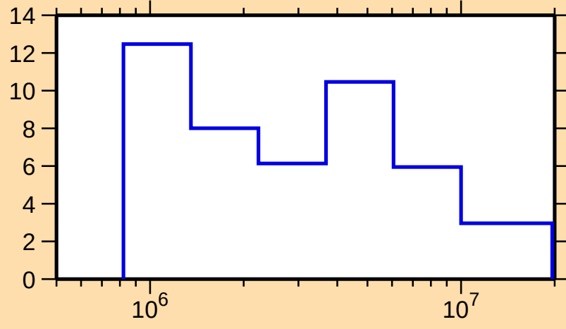
\Delta\sigma/\sigma vs. E for ^{167}\text{Dy}(n,\text{tot.})
