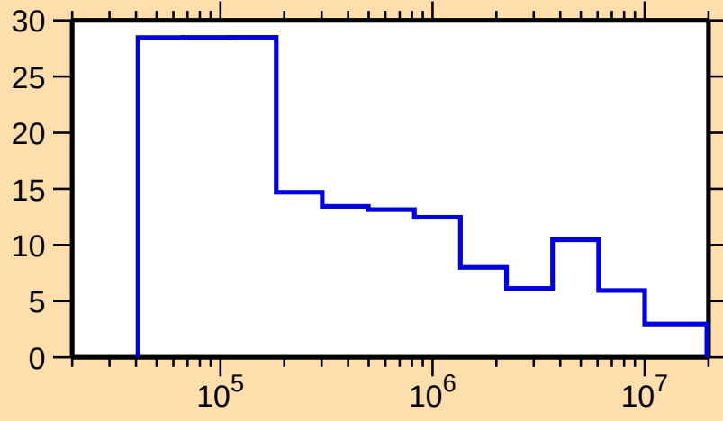
\Delta\sigma/\sigma vs. E for ^{167}\text{Dy}(n,\text{tot.})
