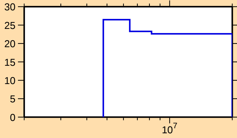
\Delta\sigma/\sigma vs. E for ^{167}\text{Dy}(n,\text{inel.})
