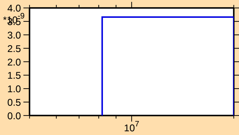
\sigma vs. E for ^{167}\text{Dy}(n,nd)
