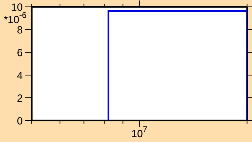
\sigma vs. E for ^{167}\text{Dy}(n,np)
