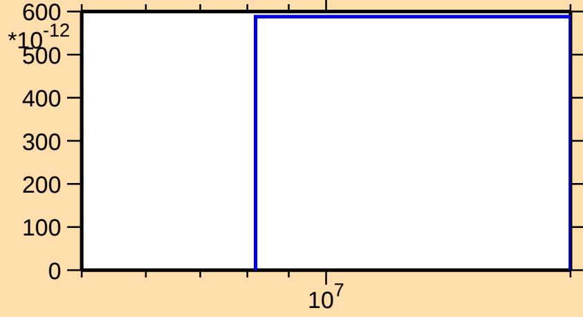
\sigma vs. E for ^{167}\text{Dy}(n,2n\alpha)
