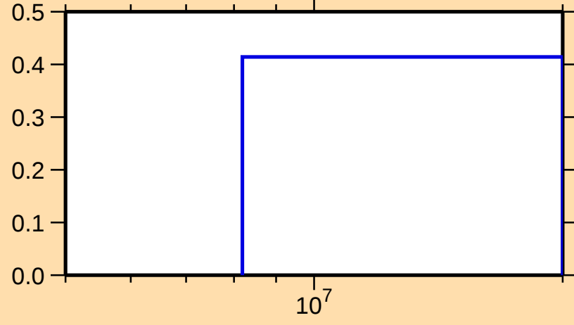
\sigma vs. E for ^{167}\text{Dy}(n,3n)
