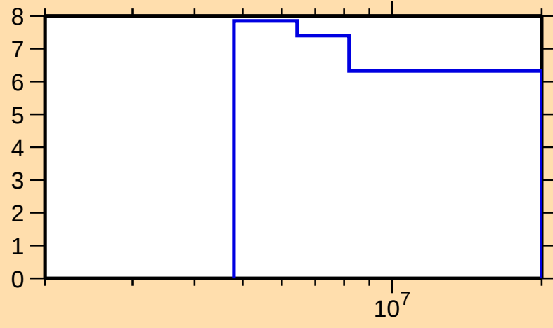
\Delta\sigma/\sigma vs. E for ^{167}\text{Dy}(n,\text{nonel.})
