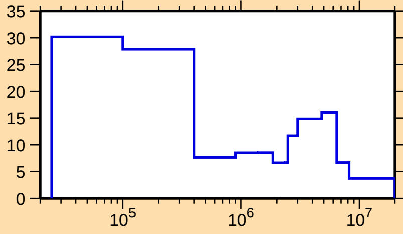
\Delta\sigma/\sigma vs. E for ^{167}\text{Dy}(n,\text{el.})
