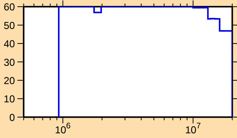
\Delta\sigma/\sigma vs. E for ^{257}\text{Es}(n,n_1)
