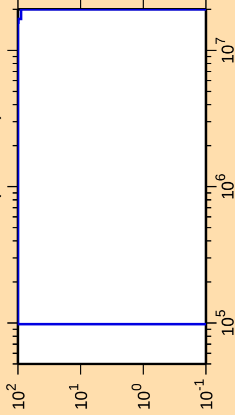
\Delta\sigma/\sigma vs. E for ^{257}\text{Es}(n,n_{\text{cont}})
