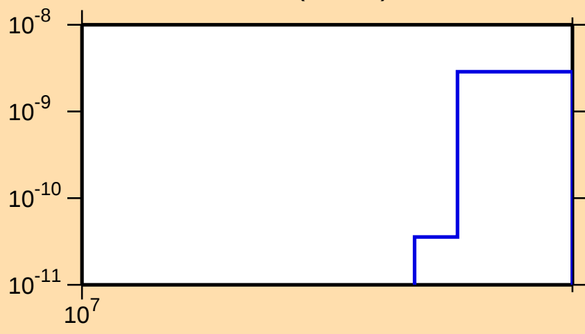
\sigma vs. E for ^{257}\text{Es}(n,3n\alpha)
