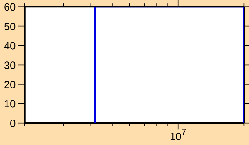
\Delta\sigma/\sigma vs. E for ^{257}\text{Es}(n,\gamma)
