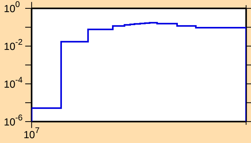
\sigma vs. E for ^{257}\text{Es}(n,3n)
