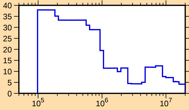
\Delta\sigma/\sigma vs. E for ^{257}\text{Es}(n,\text{tot.})
