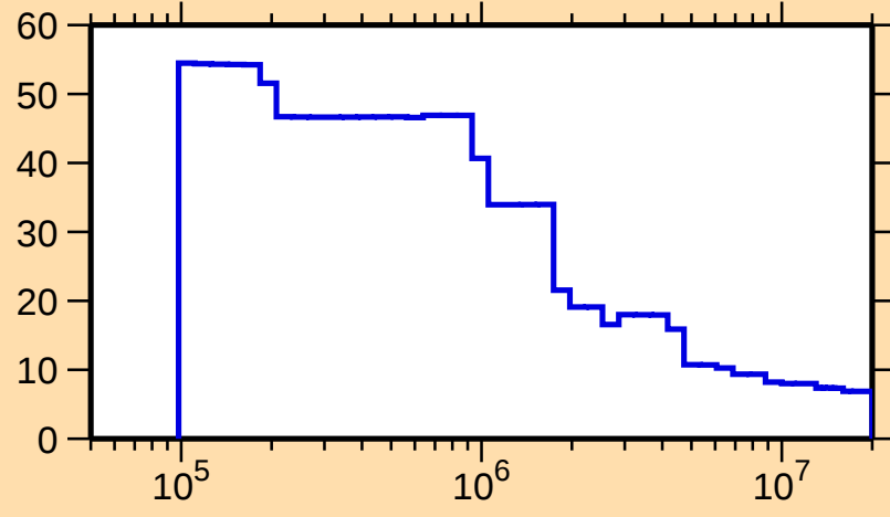
\Delta\sigma/\sigma vs. E for ^{257}\text{Es}(n,n\text{onel.})
