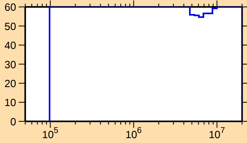
\Delta\sigma/\sigma vs. E for ^{257}\text{Es}(n,\text{inel.})
