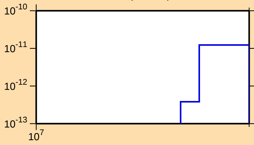
\sigma vs. E for ^{257}\text{Es}(n,\text{He3})
