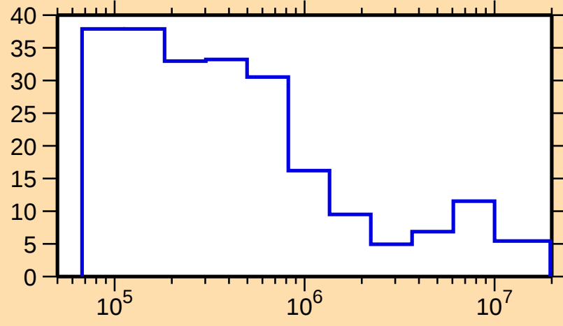
\Delta\sigma/\sigma vs. E for ^{257}\text{Es}(n,\text{tot.})
