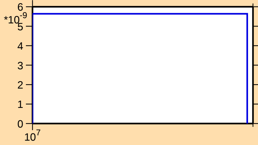
\sigma vs. E for ^{257}\text{Es}(n,2np)
