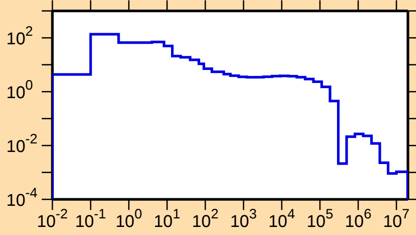
\sigma vs. E for ^{257}\text{Es}(n,\gamma)
