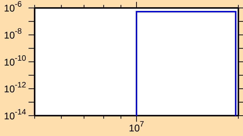
\sigma vs. E for ^{257}\text{Es}(n,nt)
