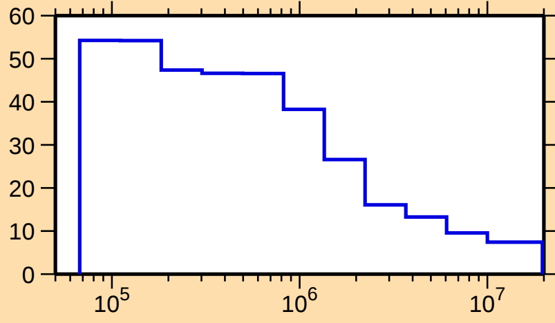
\Delta\sigma/\sigma vs. E for ^{257}\text{Es}(n,\text{nonel.})
