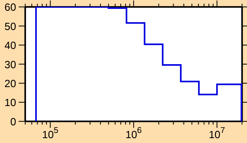
\Delta\sigma/\sigma vs. E for ^{257}\text{Es}(n,f)
