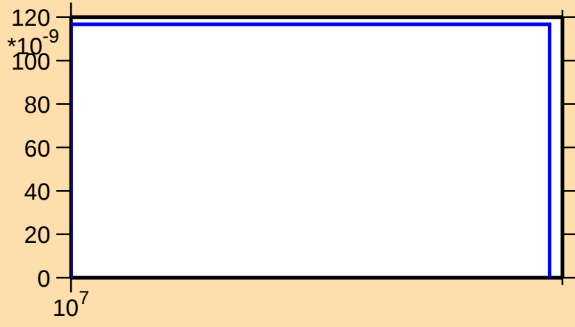
\sigma vs. E for ^{257}\text{Es}(n,\text{nd})
