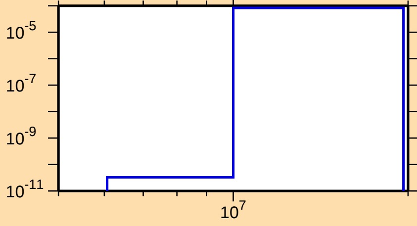
\sigma vs. E for ^{257}\text{Es}(n,t)
