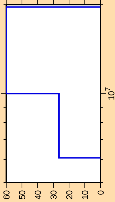
\Delta\sigma/\sigma vs. E for ^{257}\text{Es}(n,t)
