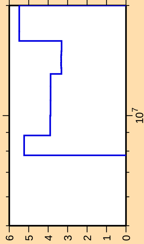
\Delta\sigma/\sigma vs. E for ^{151}\text{Eu}(n,2n)
