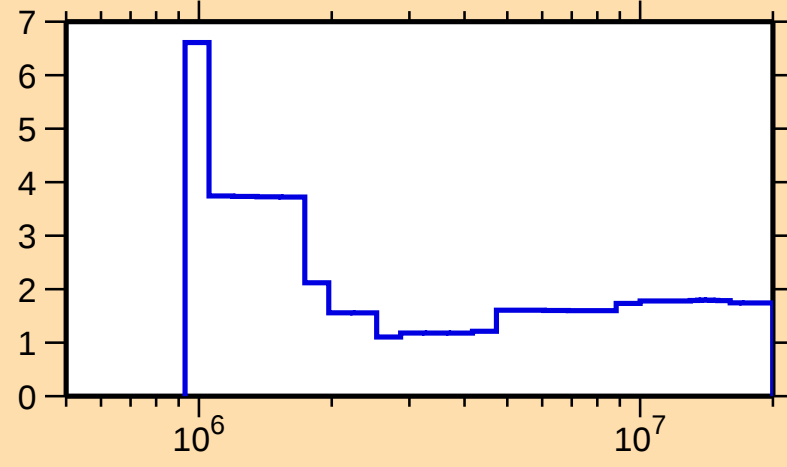
\Delta\sigma/\sigma vs. E for ^{151}\text{Eu}(n,\text{nonel.})
