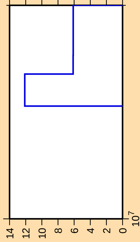
\Delta\sigma/\sigma vs. E for ^{151}\text{Eu}(n,3n)
