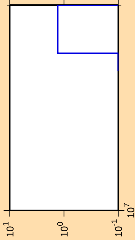
\Delta\sigma/\sigma vs. E for ^{151}\text{Eu}(n,3n\alpha)
