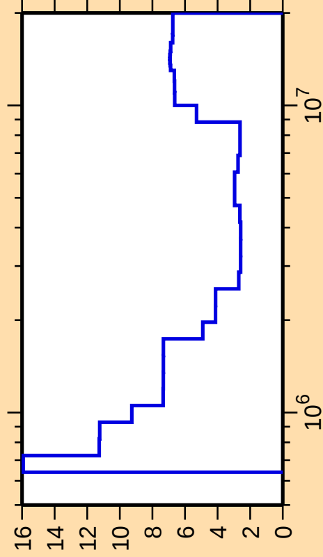
\Delta\sigma/\sigma vs. E for ^{151}\text{Eu}(n,n_{\text{cont}})
