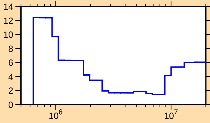
\Delta\sigma/\sigma vs. E for ^{151}\text{Eu}(n,\text{inel.})
