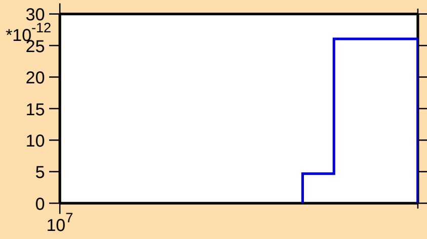
\sigma vs. E for ^{151}\text{Eu}(\text{mt117})
