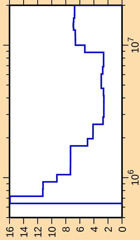
\Delta\sigma/\sigma vs. E for ^{151}\text{Eu}(n,n\text{cont.})
