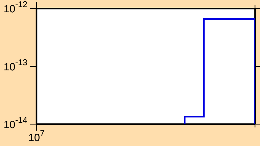
\sigma vs. E for ^{151}\text{Eu}(n,3n\alpha)
