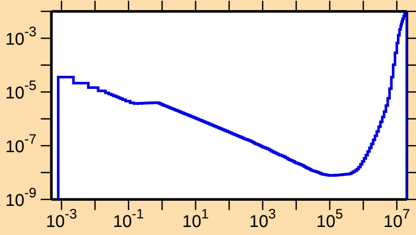
\sigma vs. E for ^{151}\text{Eu}(n,\alpha)
