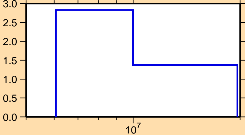
\Delta\sigma/\sigma vs. E for ^{22}\text{F}(n,2n)
