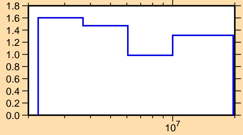
\Delta\sigma/\sigma vs. E for ^{22}\text{F}(n,\text{nonel.})
