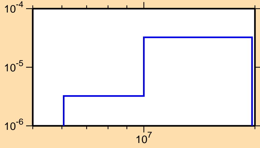
\sigma vs. E for ^{22}\text{F}(n,n\text{cont.})
