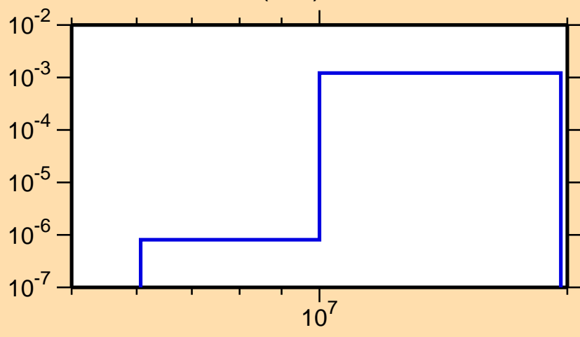
\sigma vs. E for ^{22}\text{F}(n,\alpha)
