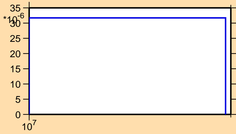
\sigma vs. E for ^{22}\text{F}(n,n\alpha)
