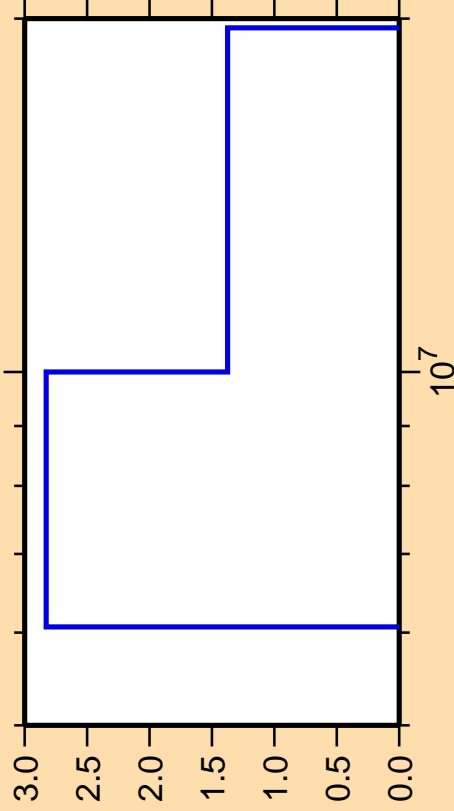
\Delta\sigma/\sigma vs. E for ^{22}\text{F}(n,2n)
