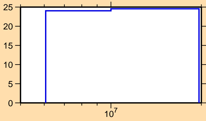
\Delta\sigma/\sigma vs. E for ^{22}\text{F}(n,ncont.)
