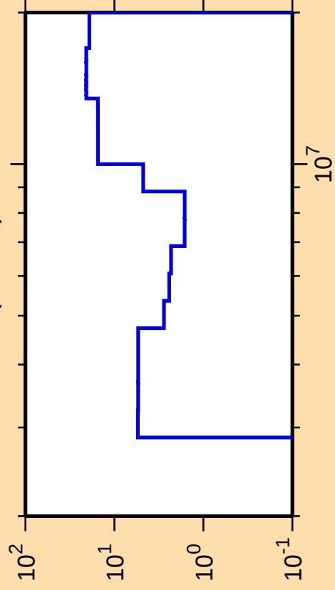
\Delta\sigma/\sigma vs. E for ^{23}\text{F}(\text{n,inel.})
