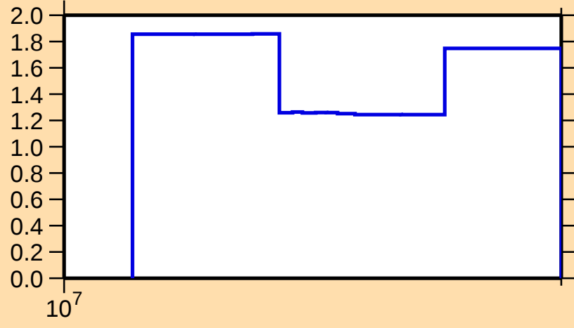
\Delta\sigma/\sigma vs. E for ^{23}\text{F}(\text{n,el.})
