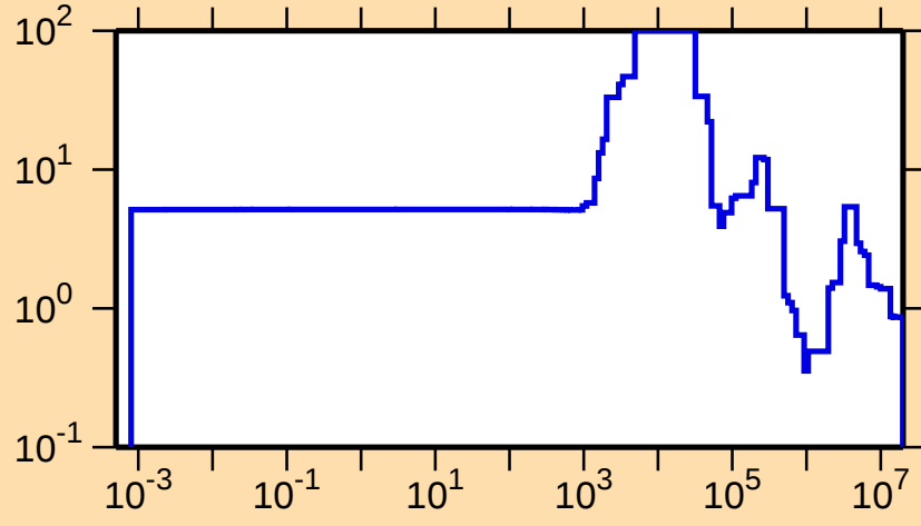
\Delta\sigma/\sigma vs. E for ^{23}\text{F}(\text{n,tot.})
