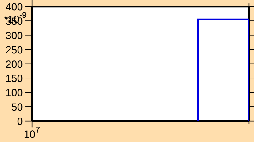
\sigma vs. E for ^{23}\text{F}(\text{n},\text{nd})
