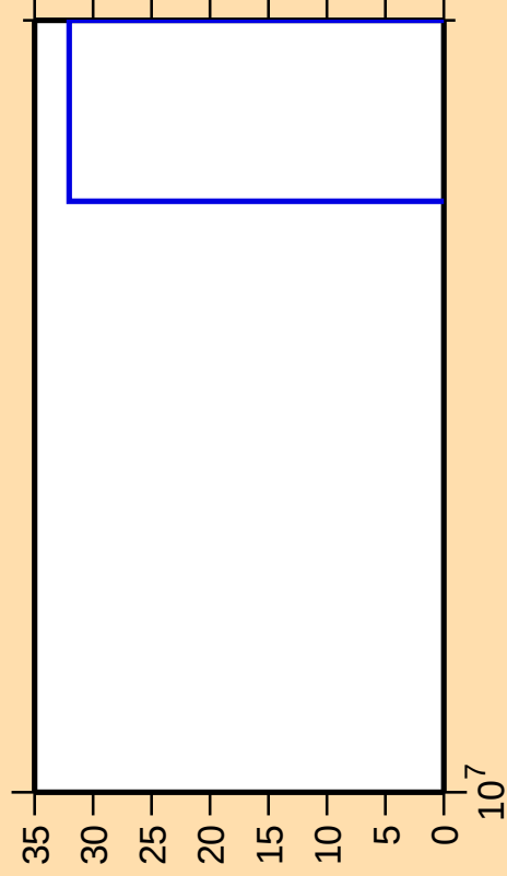
\Delta\sigma/\sigma vs. E for ^{23}\text{F}(\text{n},\text{nd})
