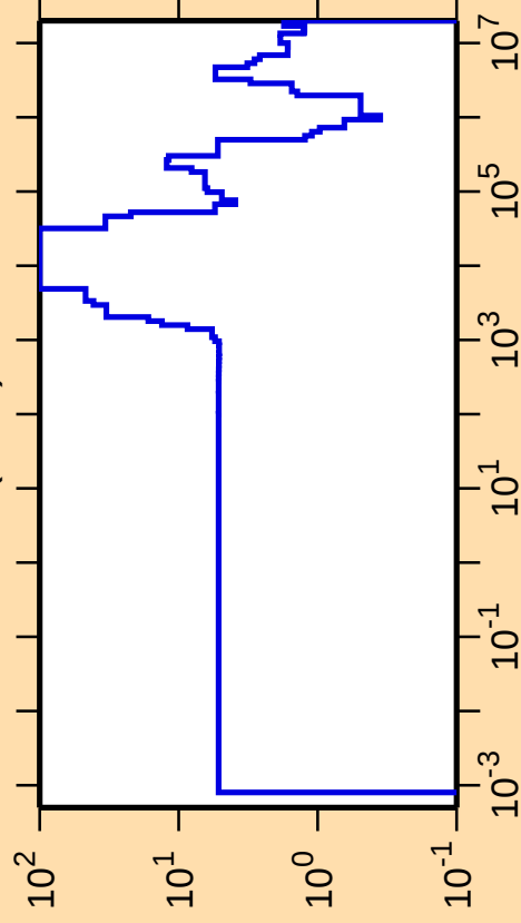
\Delta\sigma/\sigma vs. E for ^{23}\text{F}(\text{n,el.})
