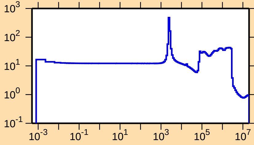
\sigma vs. E for ^{23}\text{F}(\text{n,el.})
