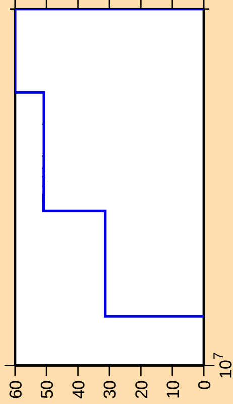
\Delta\sigma/\sigma vs. E for ^{23}\text{F}(\text{n,p})
