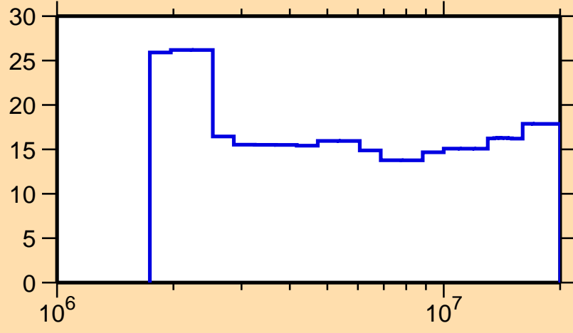
\Delta\sigma/\sigma vs. E for ^{59}\text{Fe}(n,\gamma)
