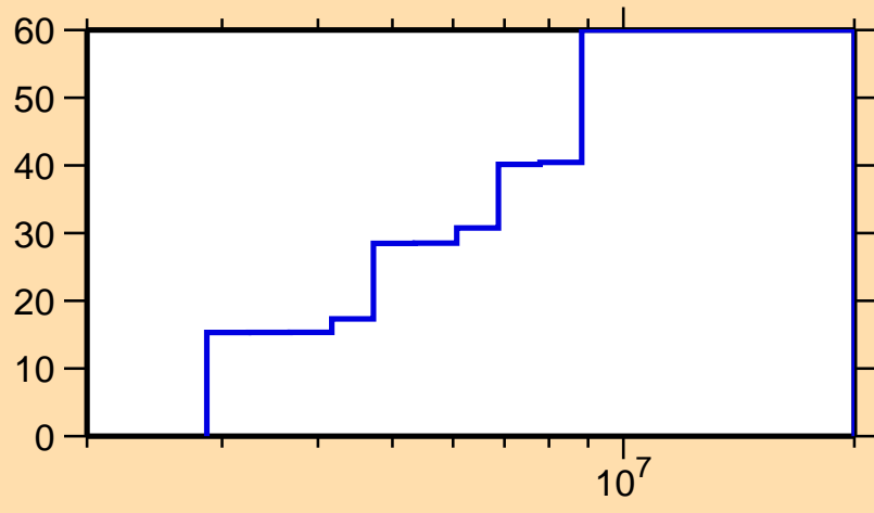
\Delta\sigma/\sigma vs. E for ^{59}\text{Fe}(n,n_1)
