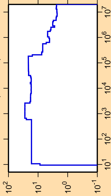
\Delta\sigma/\sigma vs. E for ^{59}\text{Fe}(n,\text{nonel.})
