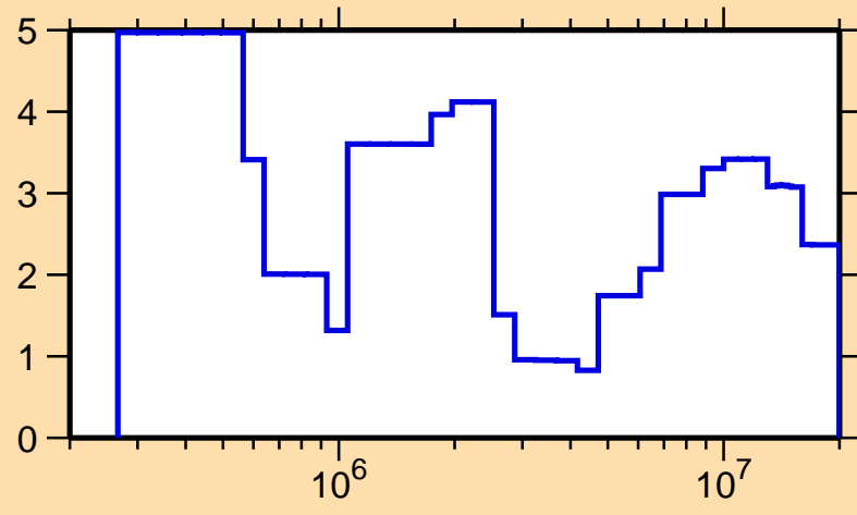
\Delta\sigma/\sigma vs. E for ^{59}\text{Fe}(n,\text{tot.})
