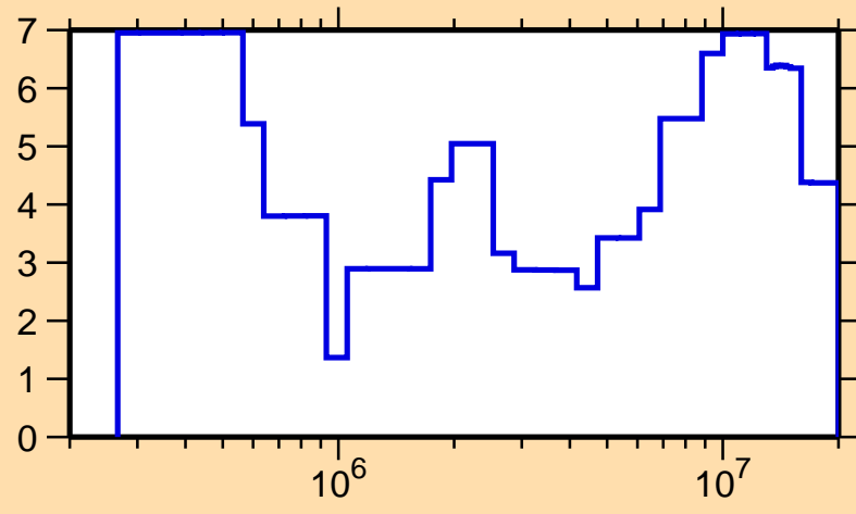
\Delta\sigma/\sigma vs. E for ^{59}\text{Fe}(n,\text{el.})
