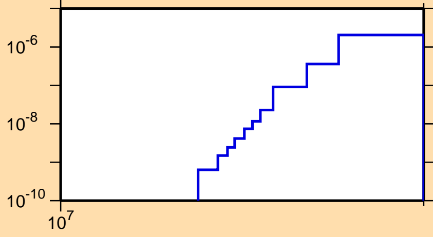
\sigma vs. E for ^{245}\text{Fm} (mt 45)
