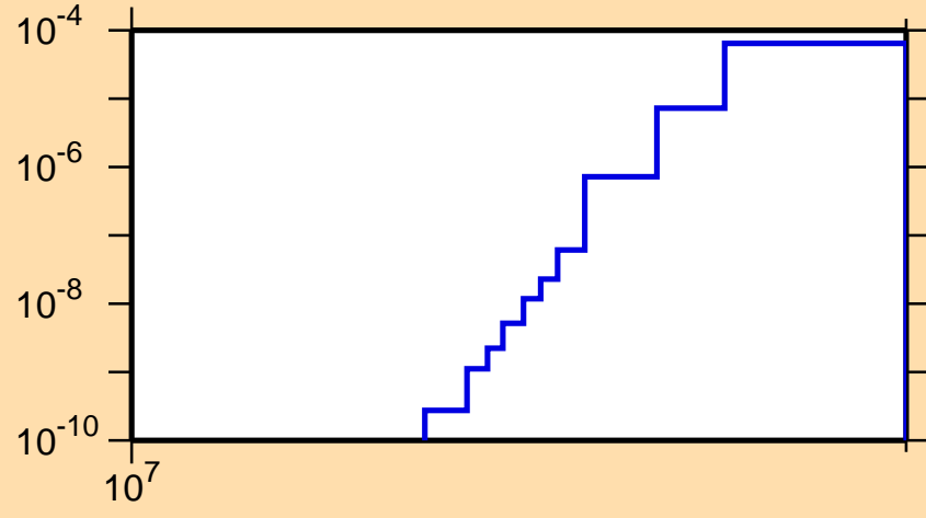
\sigma vs. E for ^{245}\text{Fm}(n,\text{nd})
