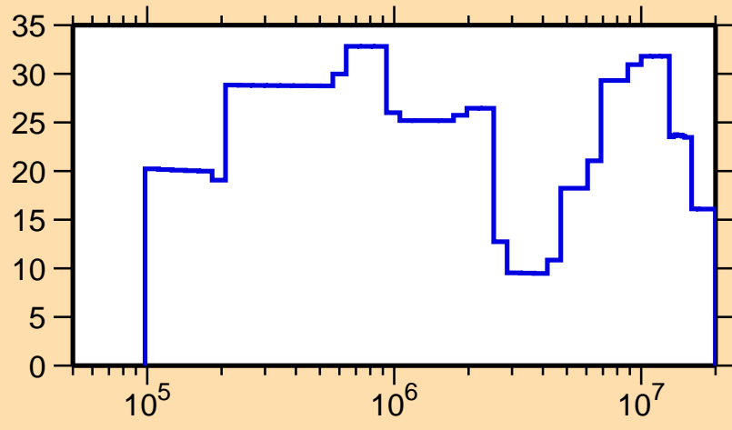
\Delta\sigma/\sigma vs. E for ^{245}\text{Fm}(n, tot.)
