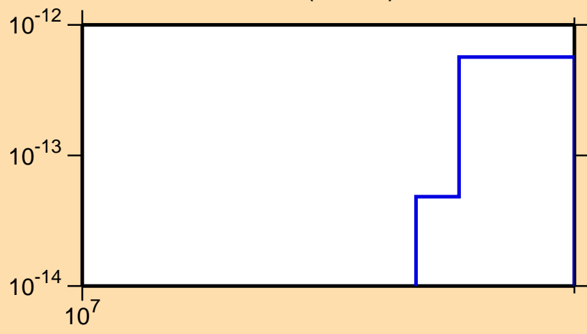
\sigma vs. E for ^{245}\text{Fm} (mt 34)
