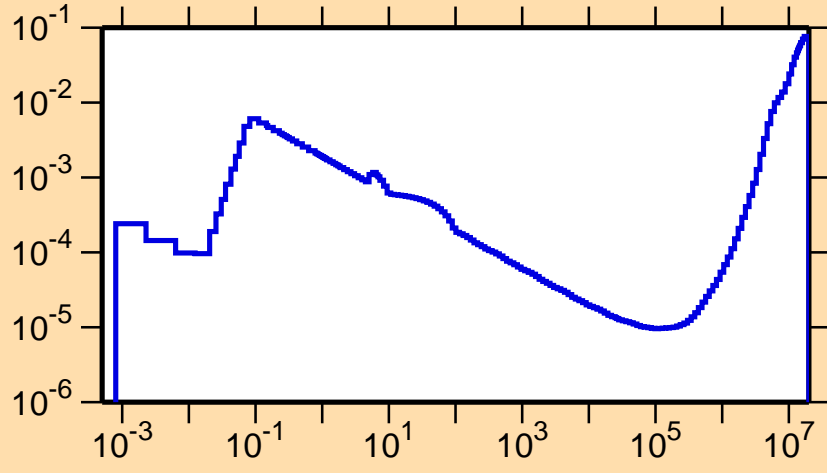
\sigma vs. E for ^{245}\text{Fm}(n,p)
