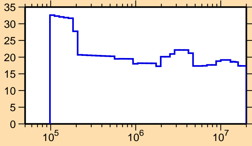
\Delta\sigma/\sigma vs. E for ^{245}\text{Fm}(n,nonel.)
