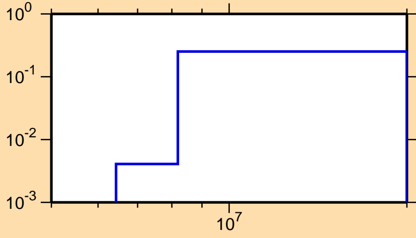
\sigma vs. E for ^{245}\text{Fm}(n,2n)
