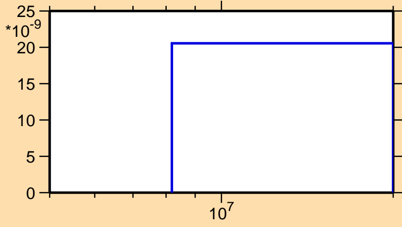
\sigma vs. E for ^{245}\text{Fm}(\text{mt117})
