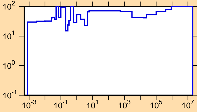
\Delta\sigma/\sigma vs. E for ^{245}\text{Fm}(n,\gamma)
