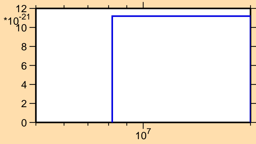
\sigma vs. E for ^{245}\text{Fm} (mt 42)
