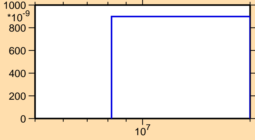
\sigma vs. E for ^{245}\text{Fm}(n,nd)
