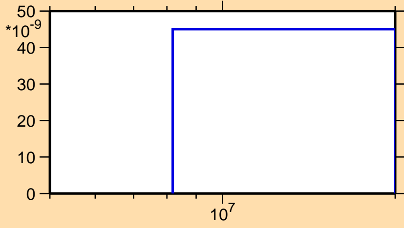
\sigma vs. E for ^{245}\text{Fm} (mt 45)
