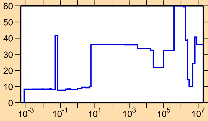
\Delta\sigma/\sigma vs. E for ^{245}\text{Fm}(n,el.)
