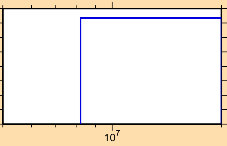
\sigma vs. E for ^{245}\text{Fm} (mt 34)
