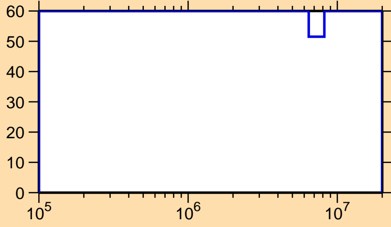
\Delta\sigma/\sigma vs. E for ^{245}\text{Fm}(n,\text{inel.})
