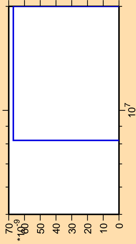
\Delta\sigma/\sigma vs. E for ^{245}\text{Fm} (mt 42)
