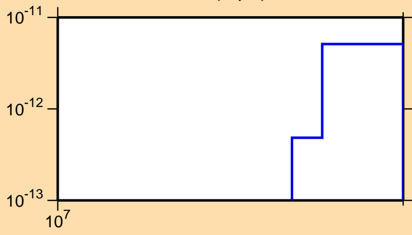
\sigma vs. E for ^{246}\text{Fm}(n,\text{pd})
