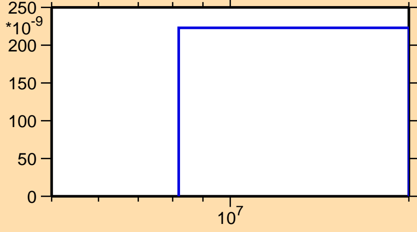
\sigma vs. E for ^{246}\text{Fm}(n,3n\alpha)
