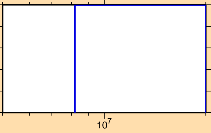
\sigma vs. E for ^{246}\text{Fm}(n,3n)
