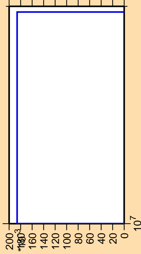
\Delta\sigma/\sigma vs. E for ^{247}\text{Fm} (mt 45)
