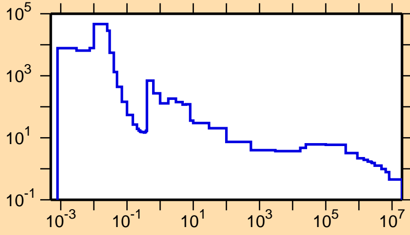
\sigma vs. E for ^{247}\text{Fm}(n,f)
