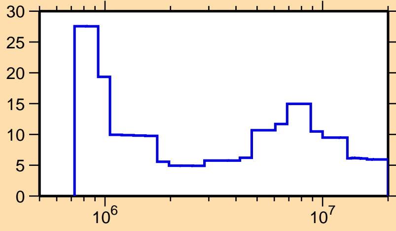
\Delta\sigma/\sigma vs. E for ^{249}\text{Fm}(n, tot.)
