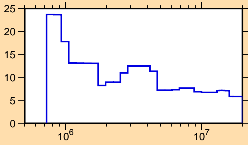
\Delta\sigma/\sigma vs. E for ^{249}\text{Fm}(n,nonel.)
