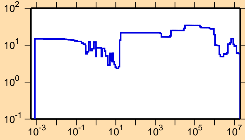
\Delta\sigma/\sigma vs. E for ^{249}\text{Fm}(n,tot.)
