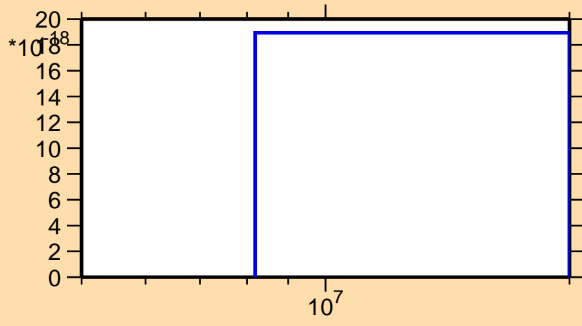
\sigma vs. E for ^{249}\text{Fm} (mt 34)
