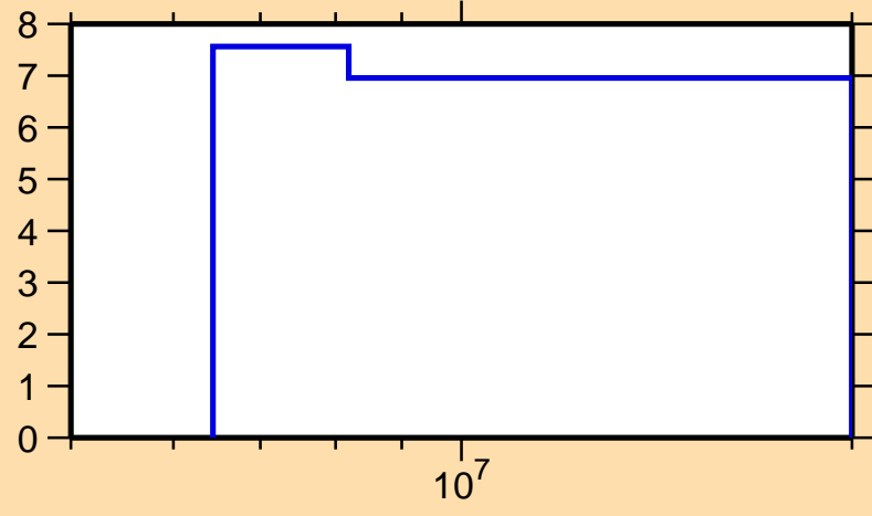
\Delta\sigma/\sigma vs. E for ^{249}\text{Fm}(n,\text{nonel.})
