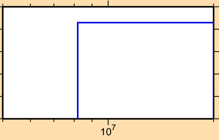
\sigma vs. E for ^{249}\text{Fm}(n,3n)
