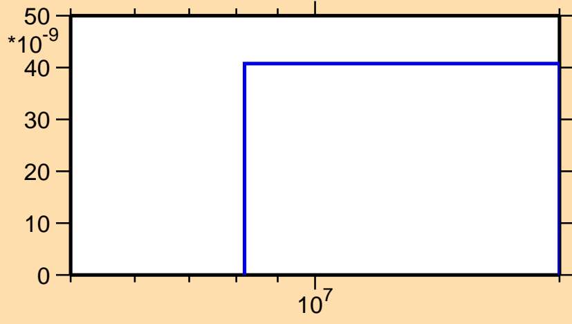
\sigma vs. E for ^{249}\text{Fm}(n,nd)
