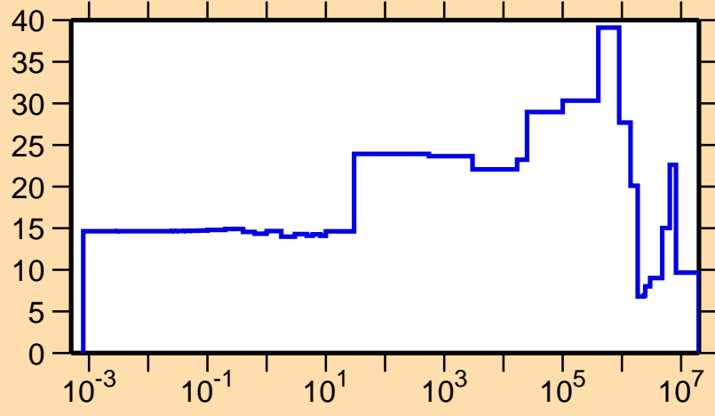
\Delta\sigma/\sigma vs. E for ^{249}\text{Fm}(n,el.)
