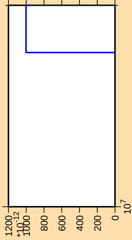
\Delta\sigma/\sigma vs. E for ^{250}\text{Fm}(\text{mt } 42)
