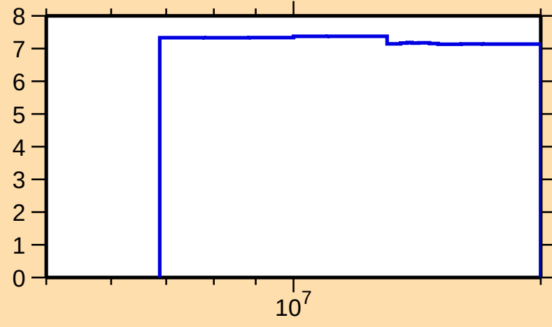
\Delta\sigma/\sigma vs. E for ^{250}\text{Fm}(n,\text{nonel.})
