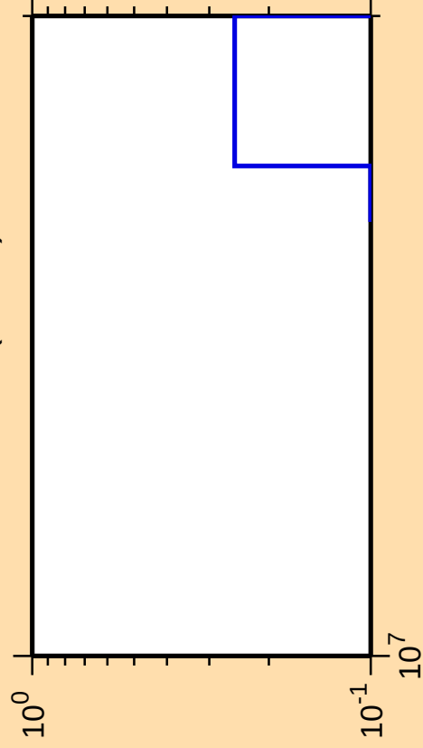
\Delta\sigma/\sigma vs. E for ^{250}\text{Fm}(\text{mt } 34)
