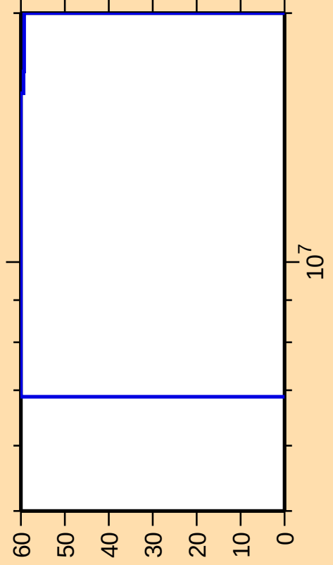
\Delta\sigma/\sigma vs. E for ^{250}\text{Fm}(n,p)
