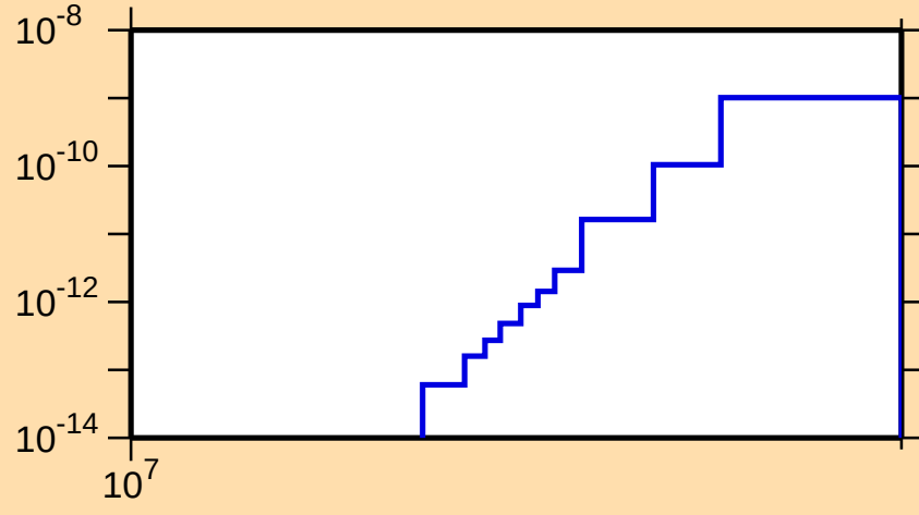
\sigma vs. E for ^{250}\text{Fm}(n,\text{He}3)
