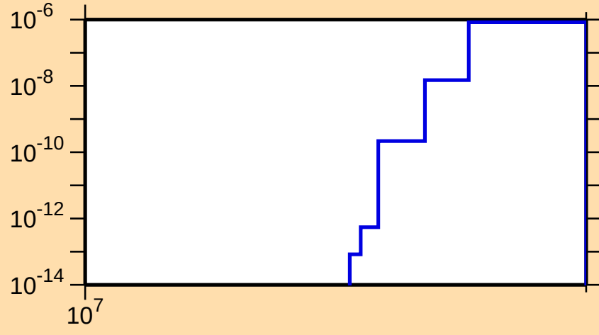
\sigma vs. E for ^{250}\text{Fm}(n,2np)
