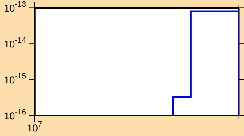
\sigma vs. E for ^{250}\text{Fm}(\text{mt } 34)
