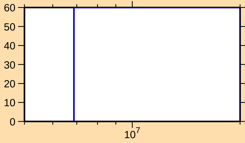
\Delta\sigma/\sigma vs. E for ^{250}\text{Fm}(n,2n)
