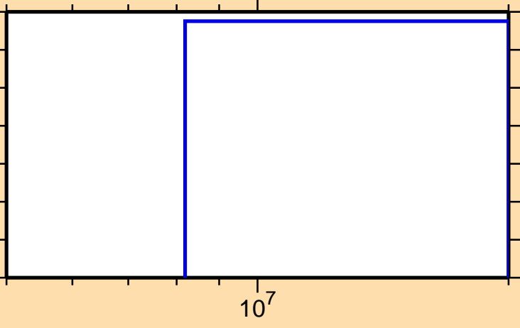
\sigma vs. E for ^{250}\text{Fm} (mt 34)
