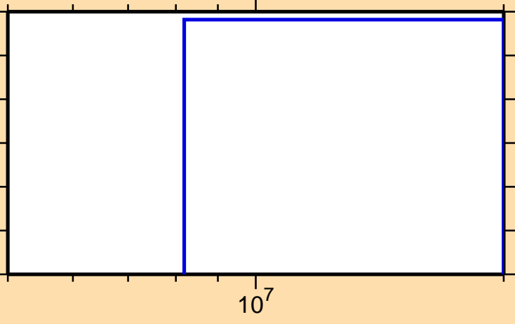
\sigma vs. E for ^{250}\text{Fm}(n,2n\alpha)
