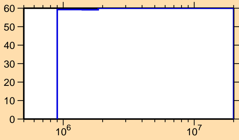
\Delta\sigma/\sigma vs. E for ^{250}\text{Fm}(n,n_1)
