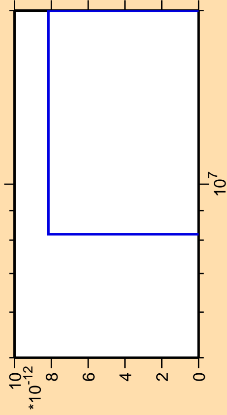
\Delta\sigma/\sigma vs. E for ^{250}\text{Fm} (mt 42)
