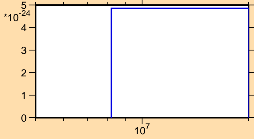
\sigma vs. E for ^{250}\text{Fm} (mt 42)
