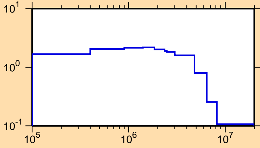
\sigma vs. E for ^{259}\text{Fm}(n,\text{inel.})
