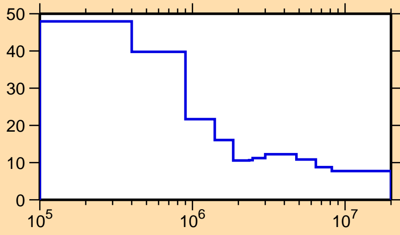
\Delta\sigma/\sigma vs. E for ^{259}\text{Fm}(n,\text{nonel.})
