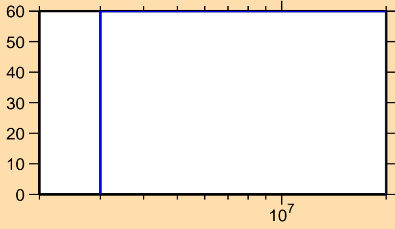
\Delta\sigma/\sigma vs. E for ^{259}\text{Fm}(n,p)
