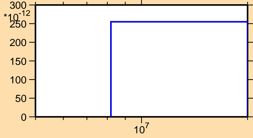
\sigma vs. E for ^{259}\text{Fm}(n,nd)
