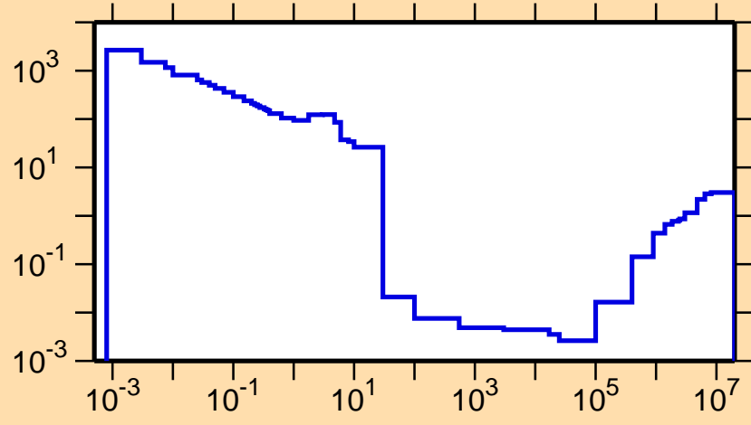
\sigma vs. E for ^{259}\text{Fm}(n,f)
