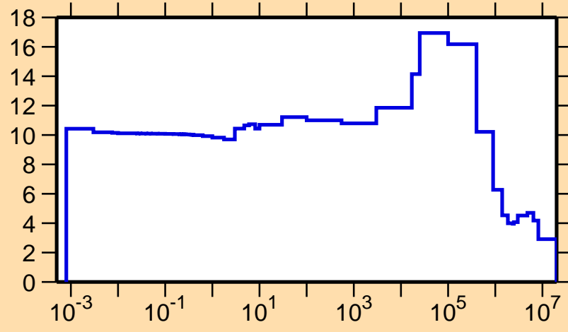
\sigma vs. E for ^{259}\text{Fm}(n,\text{el.})
