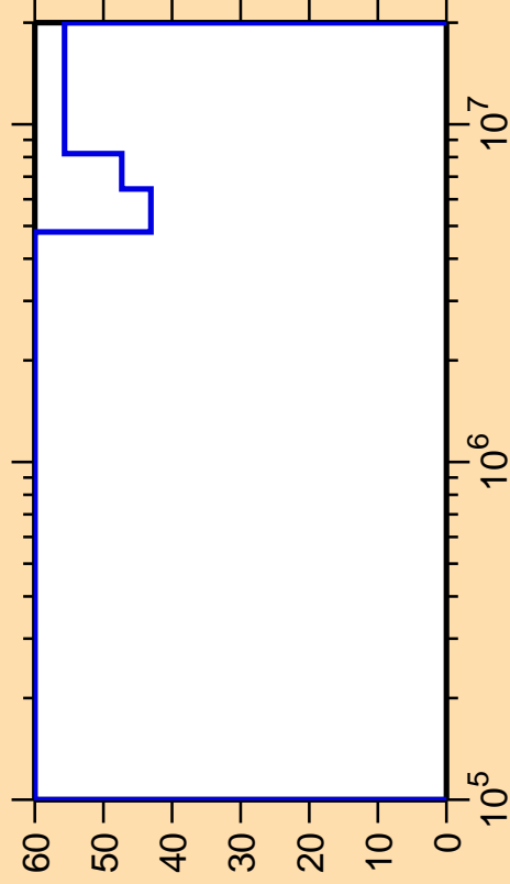
\Delta\sigma/\sigma vs. E for ^{259}\text{Fm}(n,\text{inel.})
