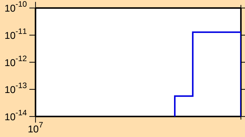
\sigma vs. E for ^{260}\text{Fm}(n,2np)
