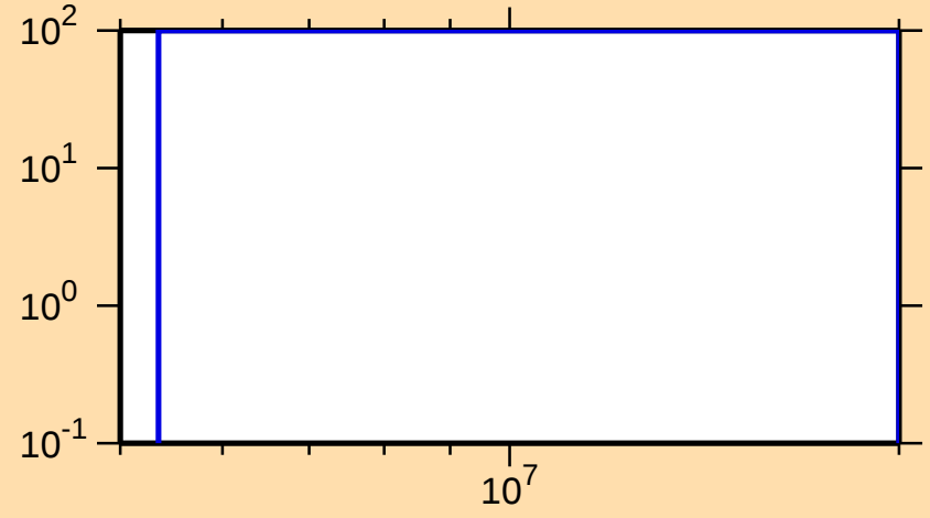
\Delta\sigma/\sigma vs. E for ^{260}\text{Fm}(n,2n)
