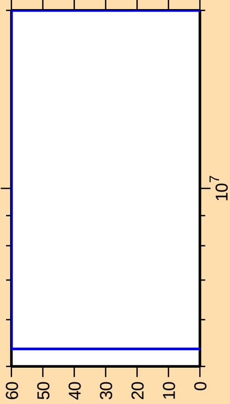
\Delta\sigma/\sigma vs. E for ^{260}\text{Fm}(n,n\text{cont.})
