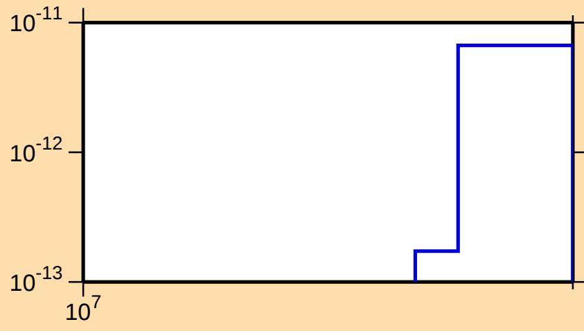
\sigma vs. E for ^{260}\text{Fm}(n,\text{He}3)
