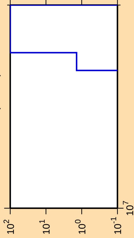
\Delta\sigma/\sigma vs. E for ^{260}\text{Fm}(n,3n\alpha)
