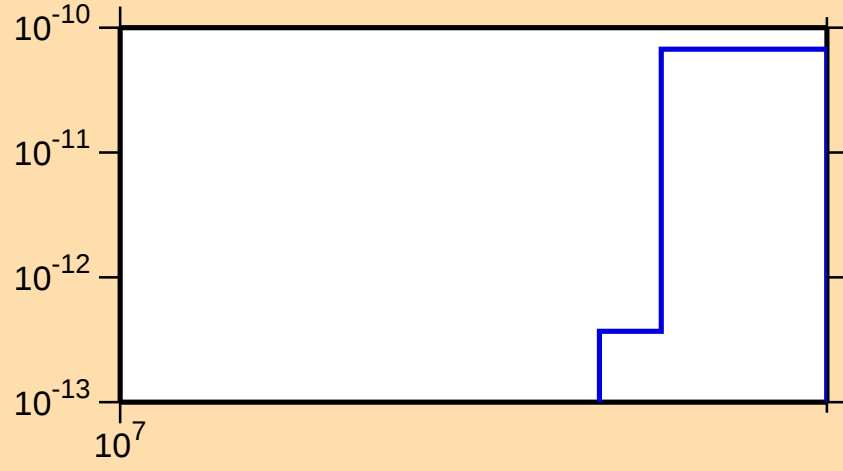
\sigma vs. E for ^{260}\text{Fm}(n,3n\alpha)
