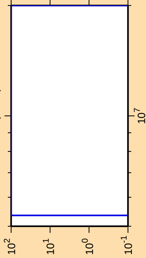
\Delta\sigma/\sigma vs. E for ^{260}\text{Fm}(n,2n)
