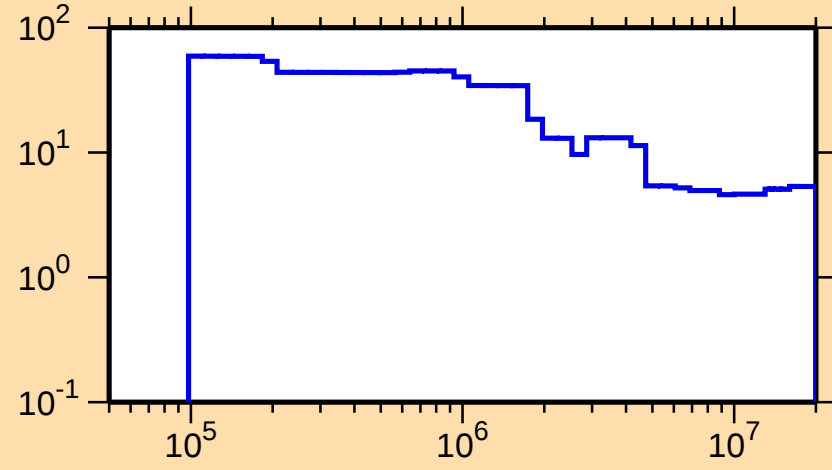
\Delta\sigma/\sigma vs. E for ^{260}\text{Fm}(n,\text{nonel.})
