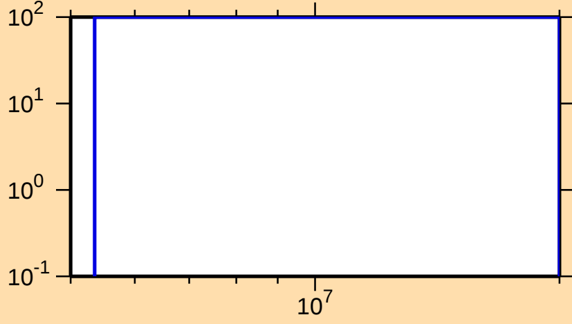
\Delta\sigma/\sigma vs. E for ^{260}\text{Fm}(n,2n)
