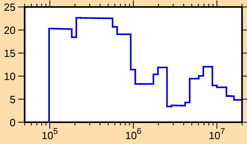
\Delta\sigma/\sigma vs. E for ^{260}\text{Fm}(n,\text{tot.})
