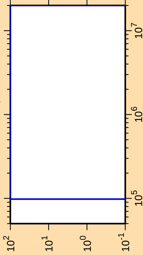
\Delta\sigma/\sigma vs. E for ^{260}\text{Fm}(n,\gamma)
