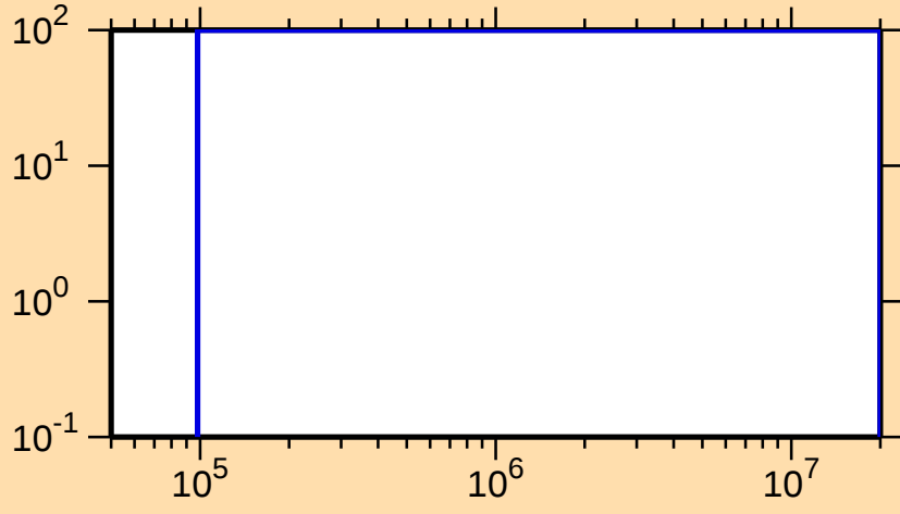
\Delta\sigma/\sigma vs. E for ^{260}\text{Fm}(n,\text{inel.})
