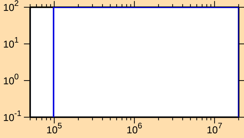
\Delta\sigma/\sigma vs. E for ^{260}\text{Fm}(n,n\text{cont.})
