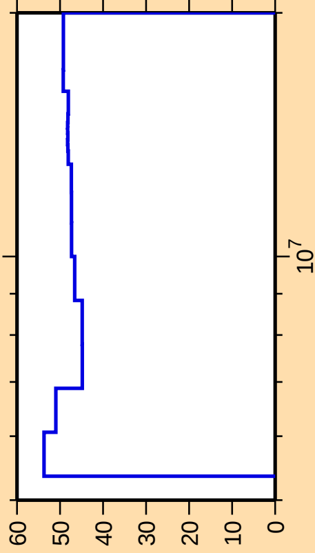
\Delta\sigma/\sigma vs. E for ^{260}\text{Fm}(n,n_1)
