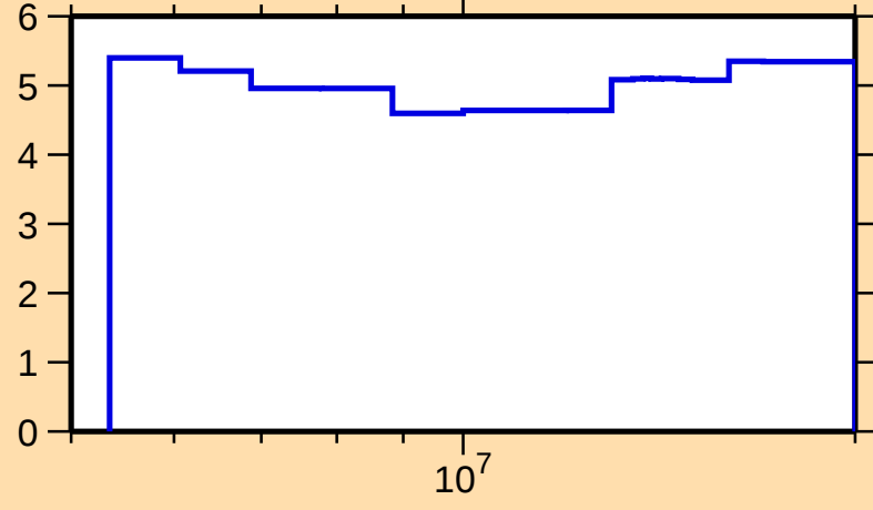
\Delta\sigma/\sigma vs. E for ^{260}\text{Fm}(n,\text{nonel.})
