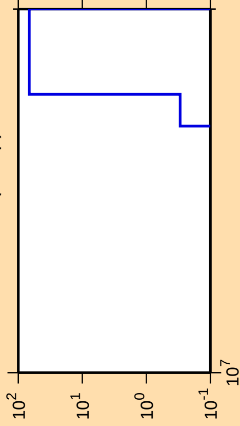
\Delta\sigma/\sigma vs. E for ^{260}\text{Fm}(n,2np)
