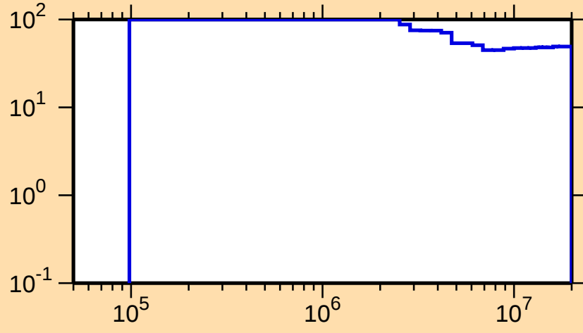
\Delta\sigma/\sigma vs. E for ^{260}\text{Fm}(n,n_1)
