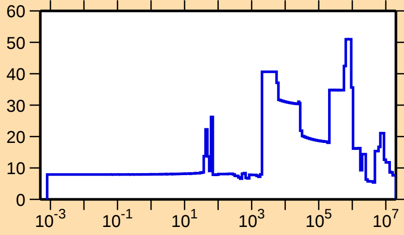
\Delta\sigma/\sigma vs. E for ^{260}\text{Fm}(n,\text{el.})
