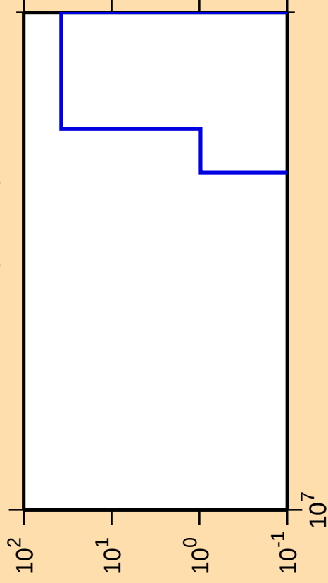
\Delta\sigma/\sigma vs. E for ^{260}\text{Fm}(n,\text{He}3)
