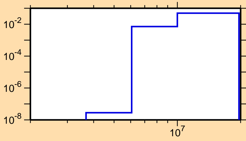
\sigma vs. E for ^{260}\text{Fm}(n,2n)
