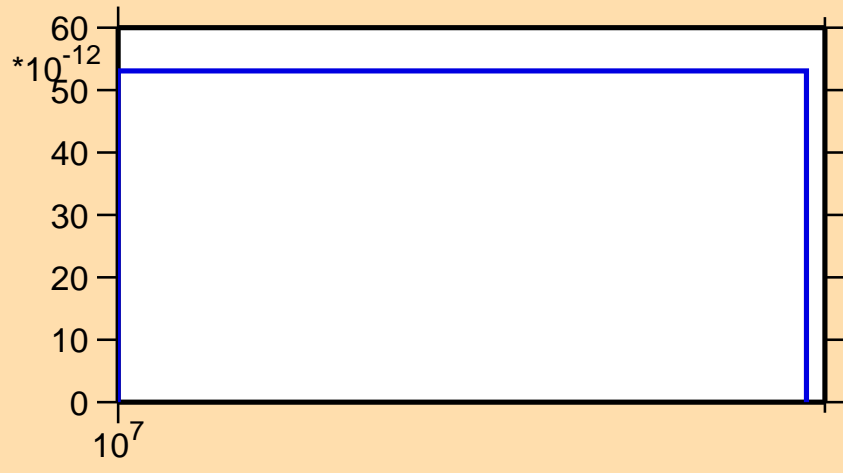
\sigma vs. E for ^{260}\text{Fm}(n,nd)
