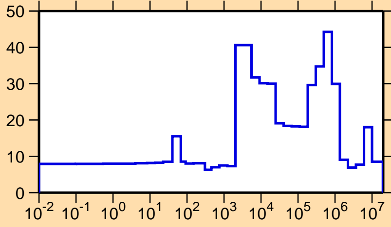
\Delta\sigma/\sigma vs. E for ^{260}\text{Fm}(n,el.)
