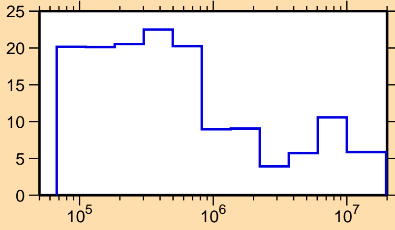
\Delta\sigma/\sigma vs. E for ^{260}\text{Fm}(n,tot.)
