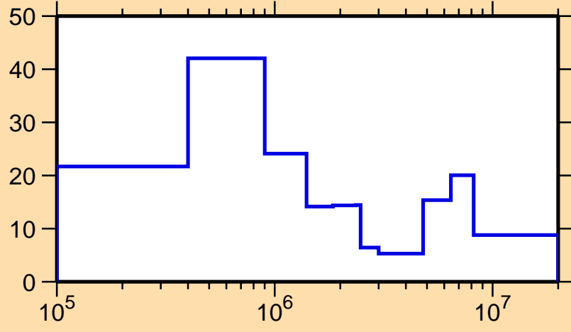
\Delta\sigma/\sigma vs. E for ^{260}\text{Fm}(n, el.)
