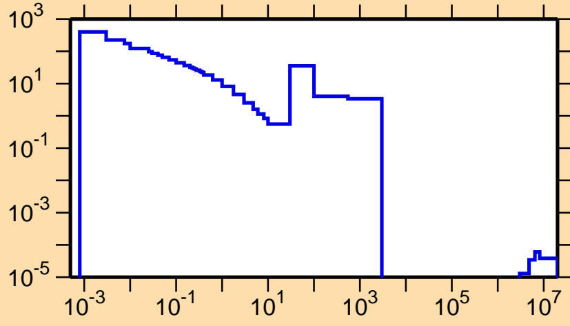
\sigma vs. E for ^{260}\text{Fm}(n,\gamma)
