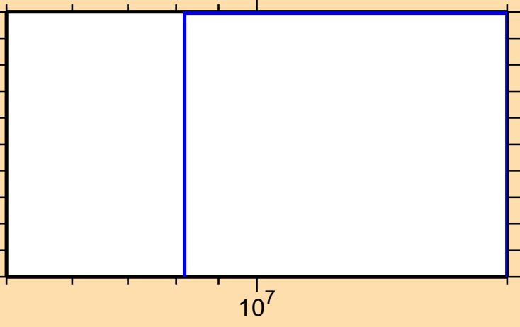
\sigma vs. E for ^{260}\text{Fm}(n,2n\alpha)
