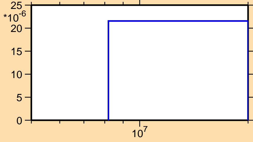
\sigma vs. E for ^{260}\text{Fm}(n,3n)
