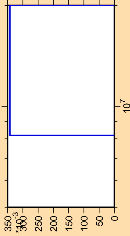
\Delta\sigma/\sigma vs. E for ^{260}\text{Fm}(n,\text{He}3)
