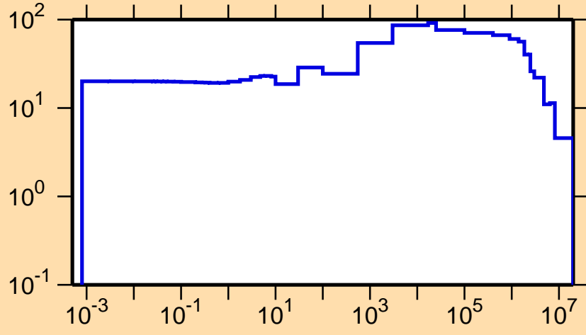
\Delta\sigma/\sigma vs. E for ^{260}\text{Fm}(n,f)
