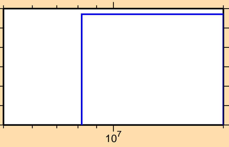
\sigma vs. E for ^{260}\text{Fm}(n,np)
